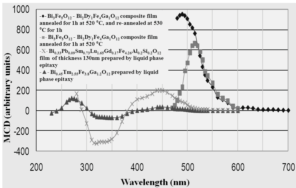
Fig. 1: Spectral dependencies of MCD signal (in arbitrary units) measured in different garnet samples. (-♦-) RF co-sputtered ( \text{Bi}_3\text{Fe}_5\text{O}_{12} - \text{Bi}_2\text{Dy}_1\text{Fe}_4\text{Ga}_1\text{O}_{12} ) composite film of thickness about 1 \mu\text{m} , annealed for 1 hour at 520°C at first stage and re-annealed for 1 hour at 530°C; (-■-) co-sputtered composite film of the same stoichiometry when still in its amorphous phase and the same thickness, but only annealed for 1 hour at 520°C; (-X-) LPE film - \text{Bi}_{0.33}\text{Pb}_{0.09}\text{Sm}_{0.73}\text{Lu}_{1.65}\text{Gd}_{0.17}\text{Fe}_{4.26}\text{Al}_{0.2}\text{Si}_{0.2}\text{O}_{12} of thickness 130 nm, and (-▲-) \text{Bi}_{0.45}\text{Tm}_{2.55}\text{Fe}_{3.8}\text{Ga}_{1.2}\text{O}_{12} film prepared by LPE. Sensitivity scale of the dichrometer was same during all measurements.
