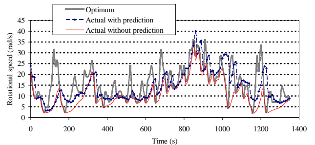
Fig. 6. Comparison performance
