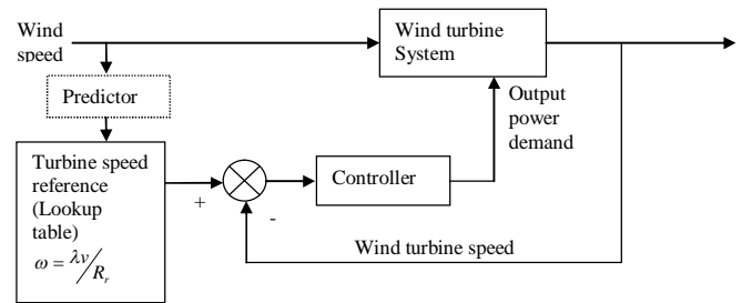
Fig. 5. Predictive control scheme with wind speed prediction
