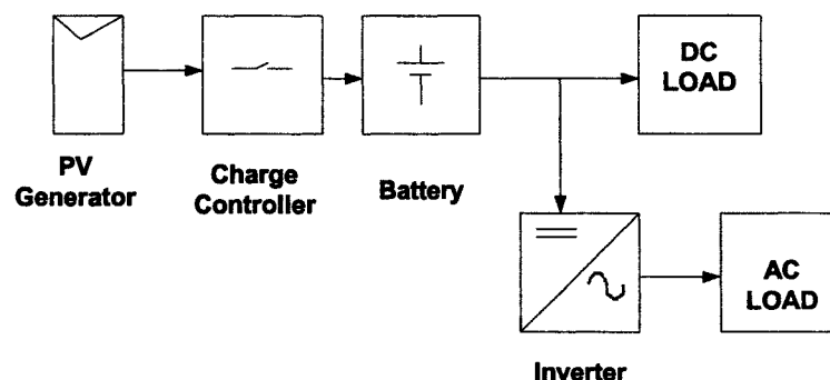
Figure 2-8 Schematic diagram of a standalone PV system
