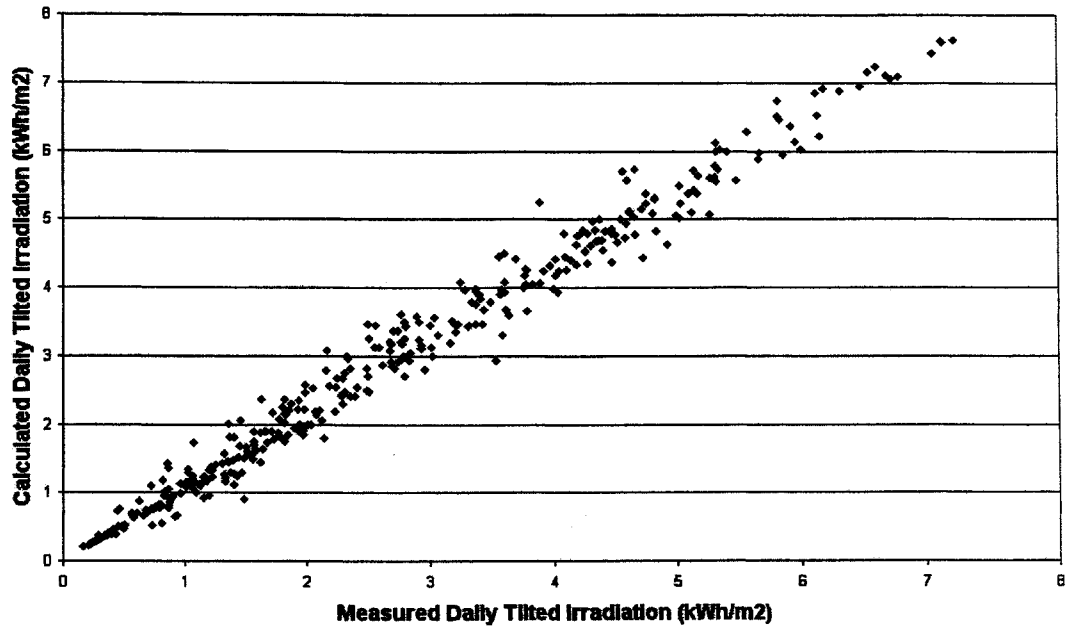
Figure 3-38 Comparison of daily total of hourly tilted irradiation for the West Midlands 1 location
