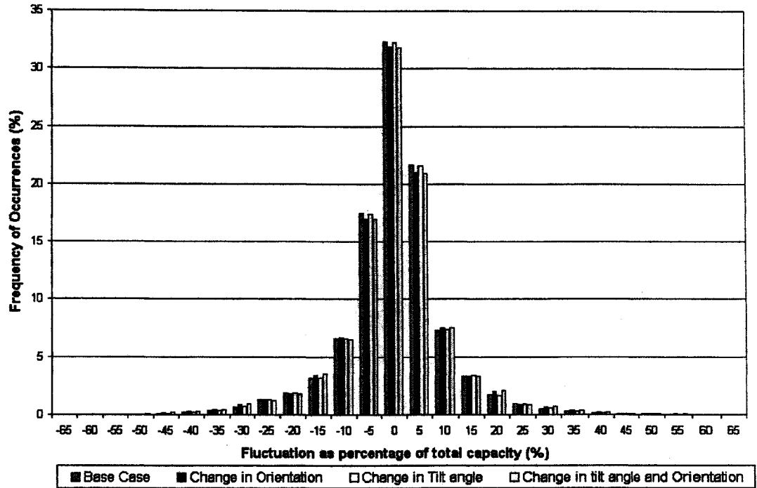
Figure 4-19 Power fluctuation pattern for the change in tilt angle and orientation
