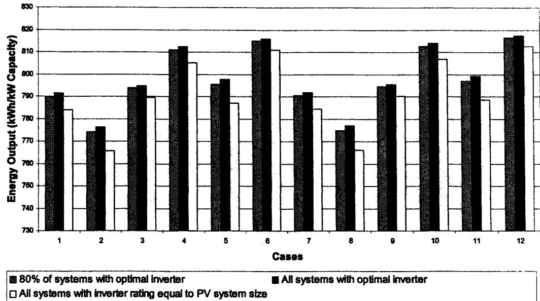
Figure 4-18 Comparison of energy output from the SMC for 12 different cases with changes in inverter ratings
