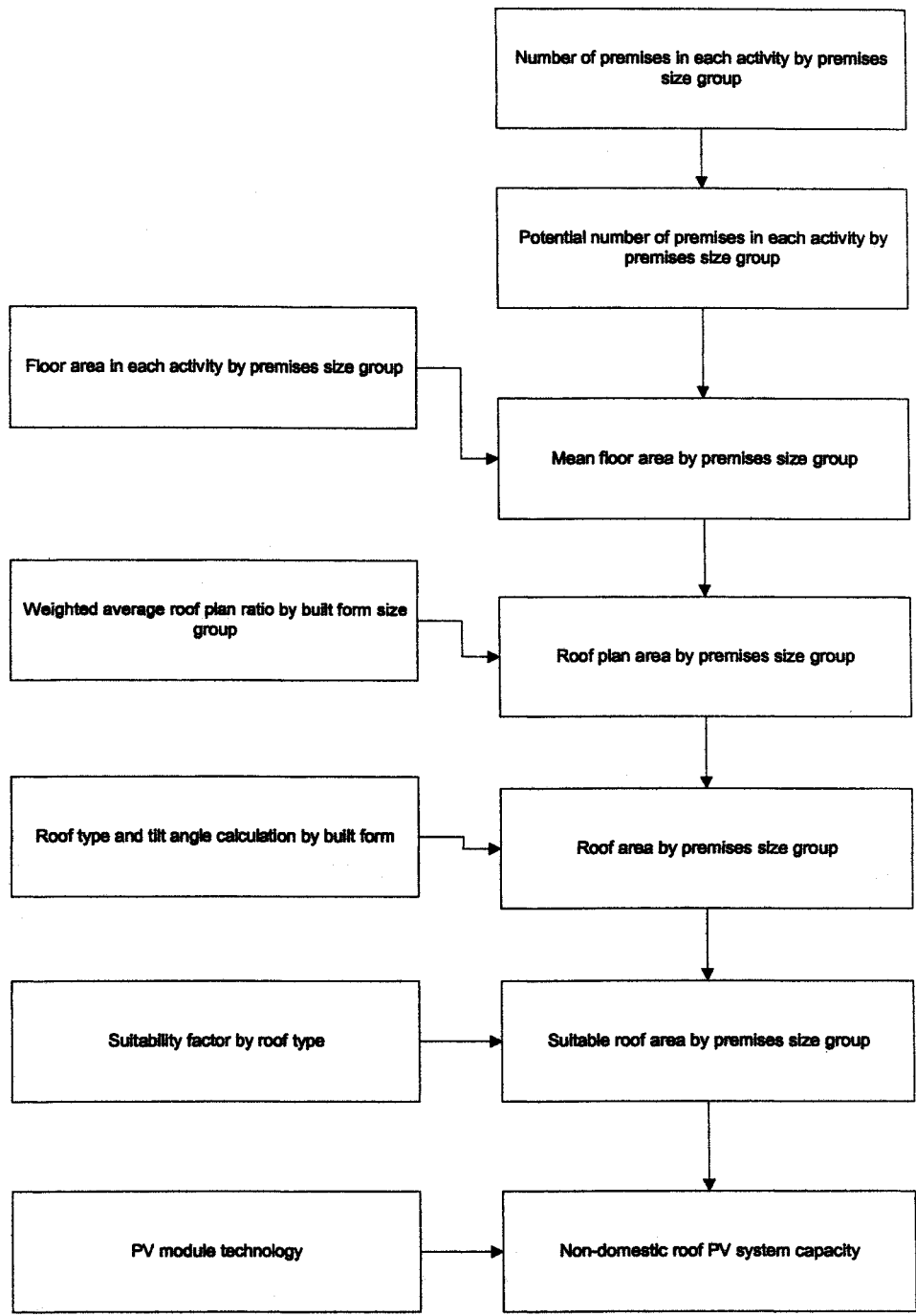
Figure 4-10 Flow chart to illustrate the non-domestic roof PV system capacity calculation
