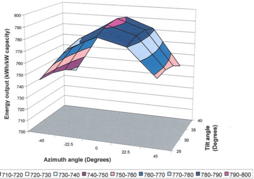
Figure 4-15 Energy output for different tilt angles and azimuth angles
