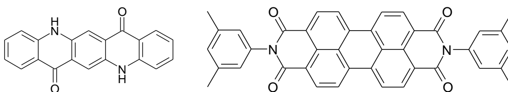
Figure 2.4 Examples of pigment structures. Left, quinacridone PV19.
