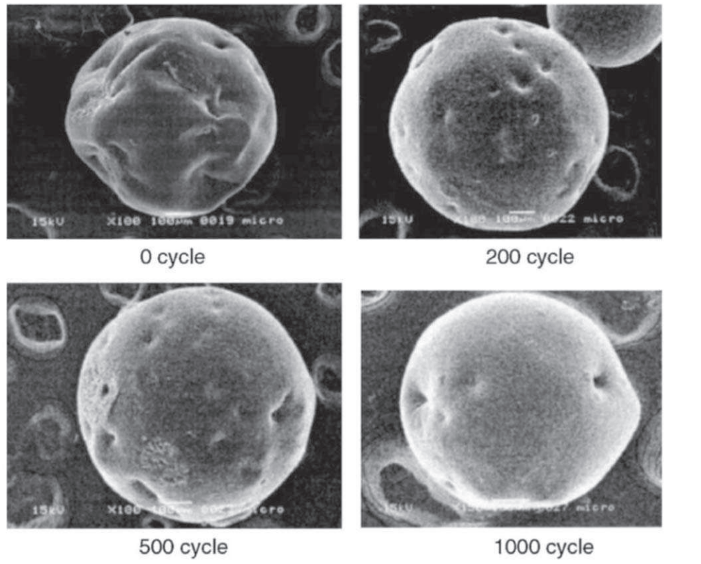
Figure 2: Microencapsulated paraffin profile evaluated by scanning electron microscope at different thermal cycles (Hawlander, Uddin and Zhu, 2002, cited by Khudair and Farid, 2004)
