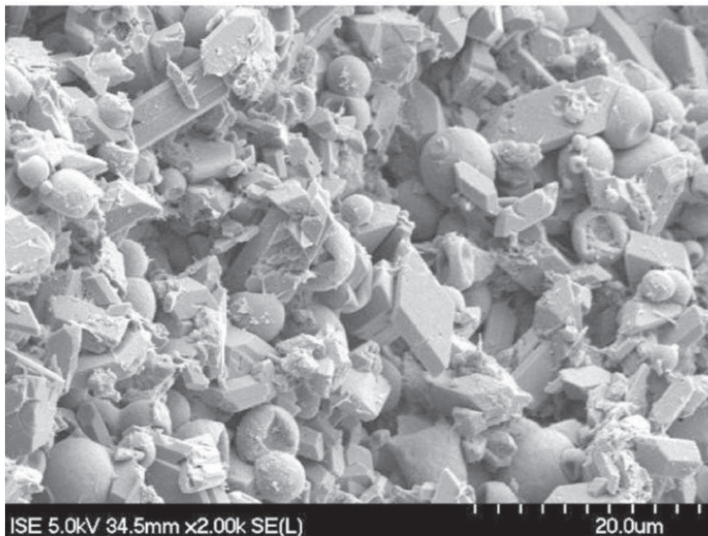
Figure 3: Scanning electron microscope image of the spherical PCM micro-capsules homogeneously dispersed between the gypsum plaster crystals (Schossig et al, 2005).
