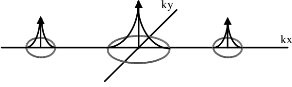
Figure 3: Spectral representation of an off-axis hologram
