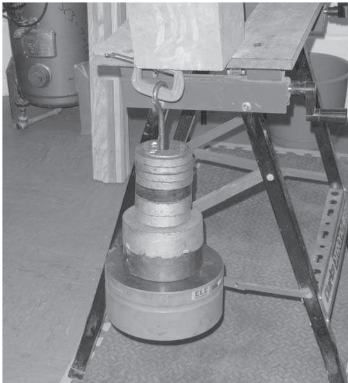
Figure 2 – Steel fibre under pull out load
