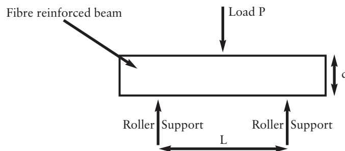
Figure 3 – Beam loading arrangement
