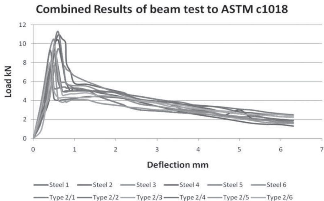
Figure 5 – Combined Results of beam test to ASTM c1018 test using Type 2 synthetic and steel fibre Reinforced Concrete – showing load and deflection
