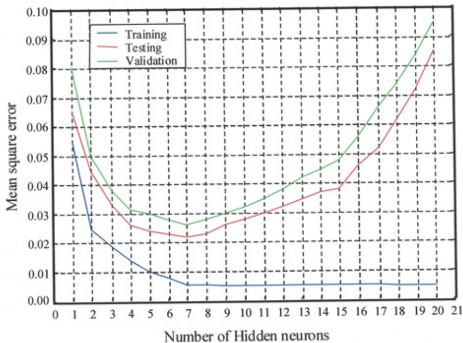
Figure (7.3): Network mean square error
