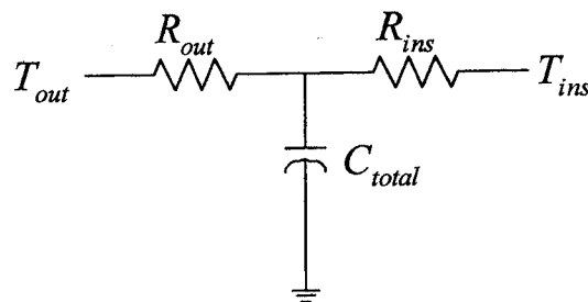
Figure (3.5): "Lumped Parameters" construction element.
