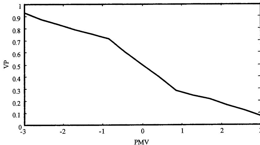
Figure (6.5): Input/output relationship for the fuzzy controller
