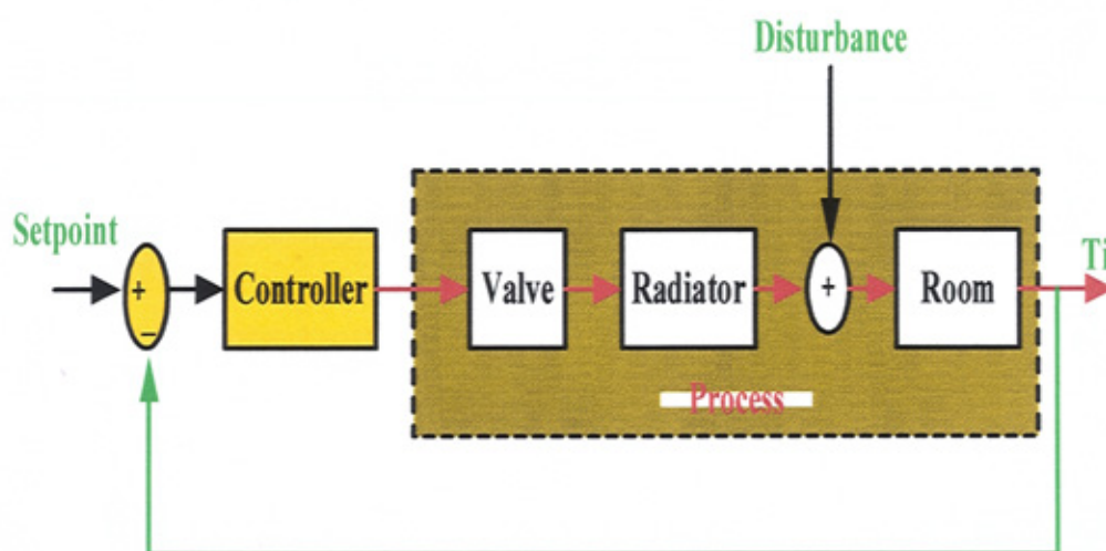
Figure (5.5): Closed loop system
