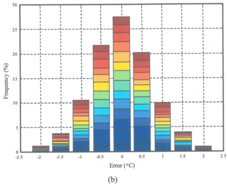
Figure (7.8): (a) Predicted internal air temperature (90 min. ahead) (b) Error distribution (90 min. ahead)
