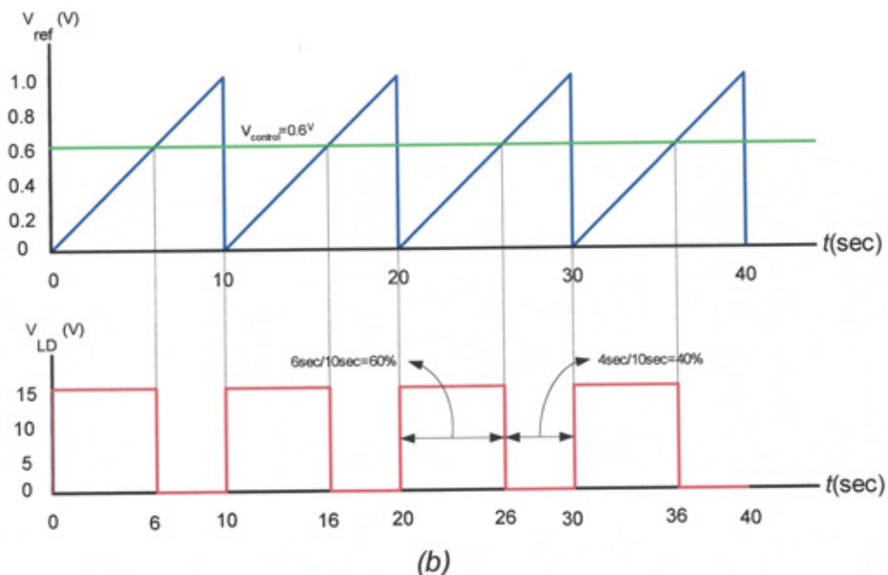
Figure (8.6): Pulse width modulation waveforms (a): Small voltage (b): Large voltage
