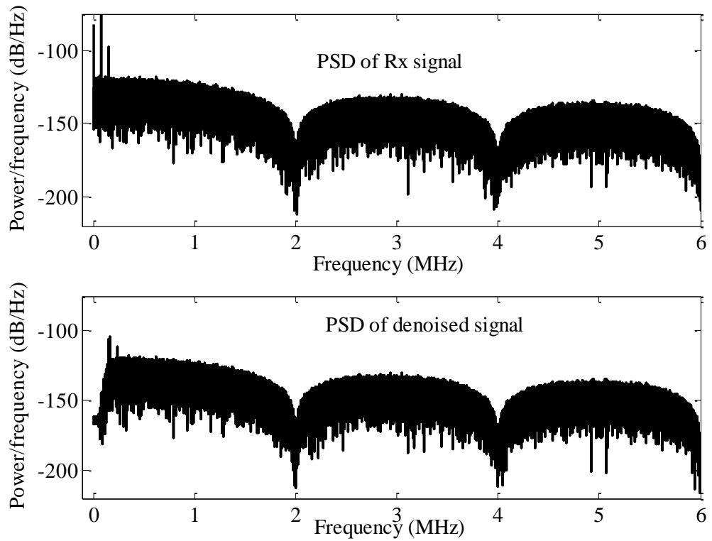
Figure 5.13 : The PSD of OOK at 2 Mbps: (a) received signal with FLI, and (b) wavelet denoising. The Daubechies wavelet with 6 levels of decompositions is used.
