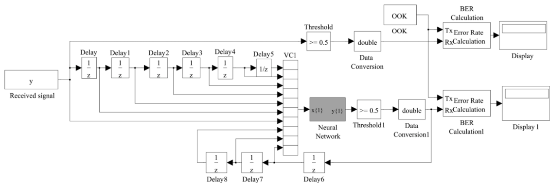
Figure 9.6 : Simulink model of ANN based DFE structure.
