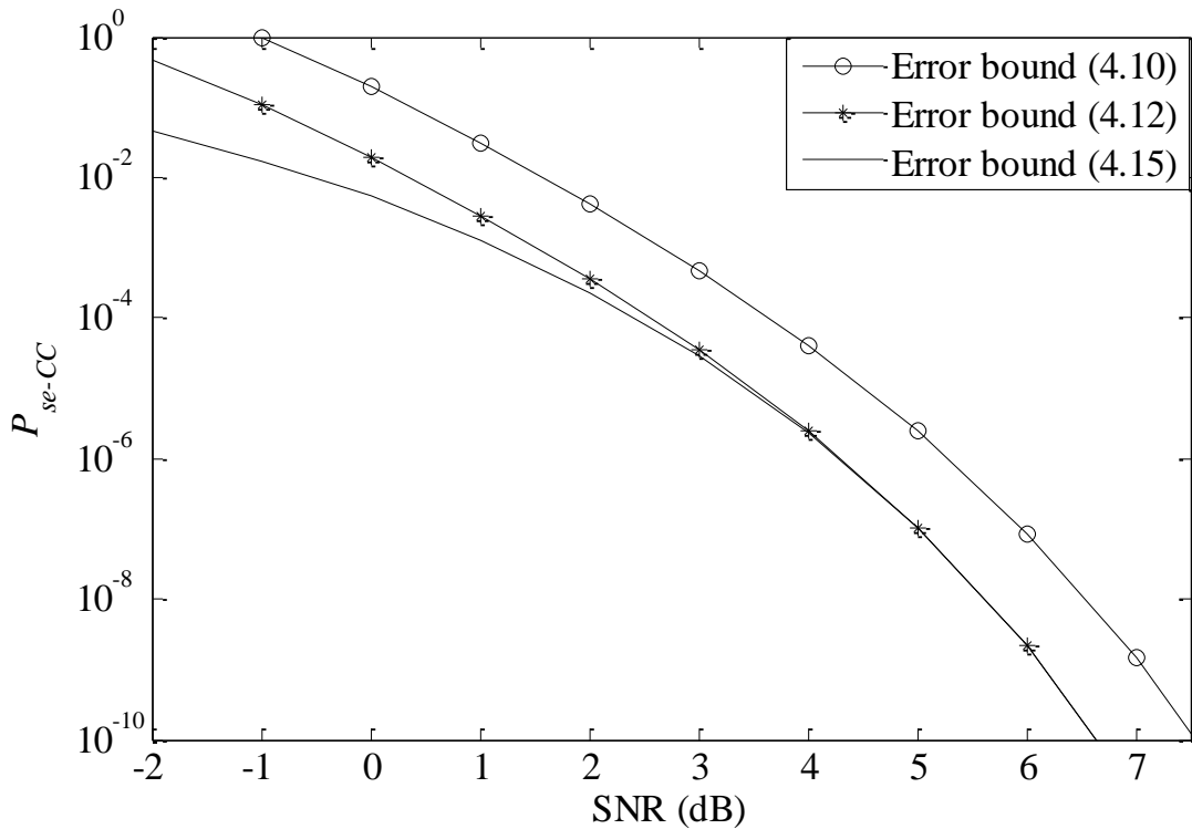
Figure 4.8: The SER against the SNR for different error bounds for CC-DH-PIM 2 .
