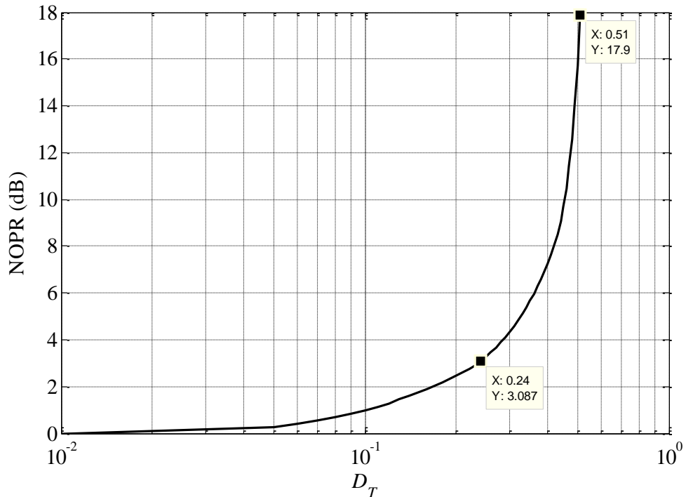
Figure 6.2: NOPR against the normalized delay spread D_T for unequalized OOK in a diffuse indoor OWC channel.
