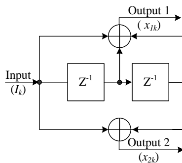
Figure 4.1: \frac{1}{2} Convolutional code encoder.
