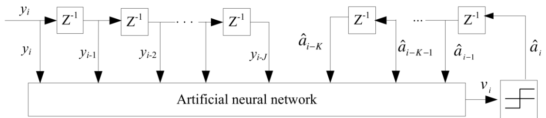
Figure 6.19: ANN based DFE structure.
