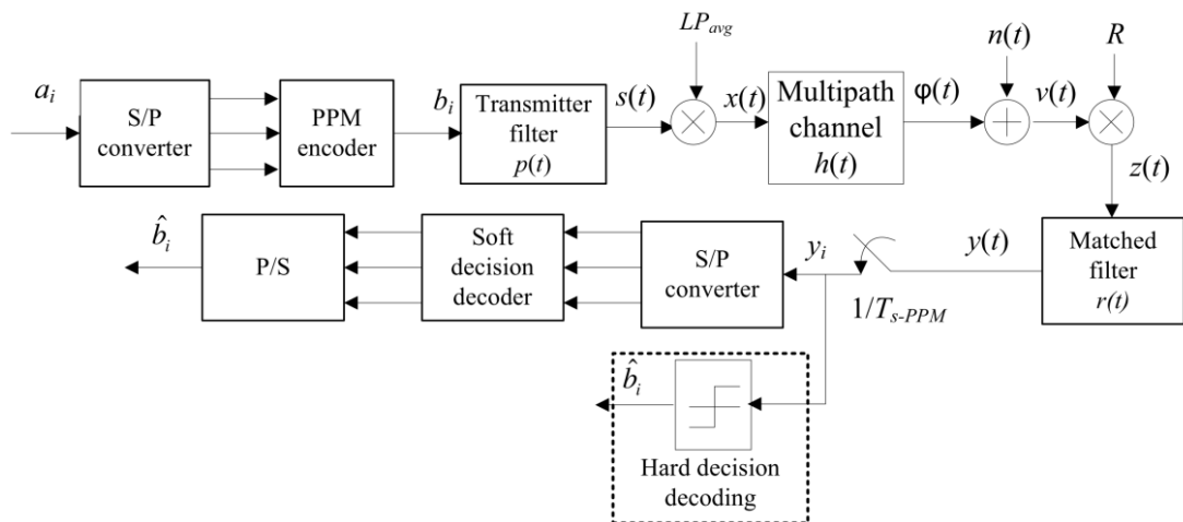
Figure 6.4: The block diagram of the unequalized PPM system with hard and soft decision decoding schemes.
