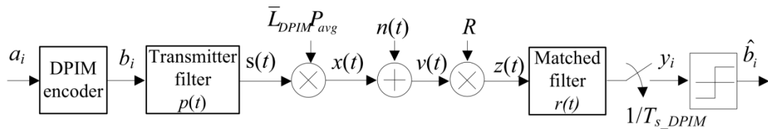
Figure 2.9: The block diagram of the matched filter based receiver for DPIM scheme.
