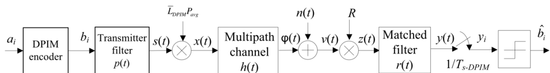
Figure 6.6: Block diagram of the unequalized DPIM system with a threshold detector.
