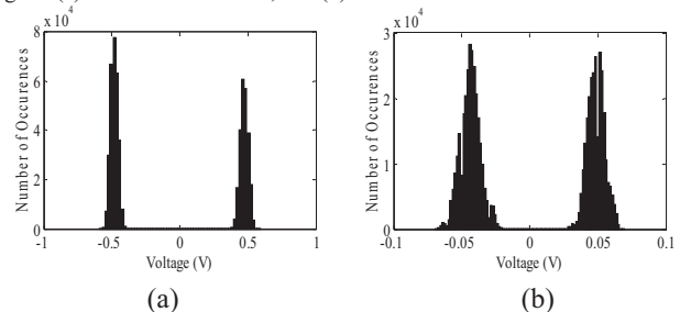
Figure A2. Received signal distribution for OOK-NRZ for a 150 mV p-p input signal: (a) without scintillation, and (b) with scintillation.
