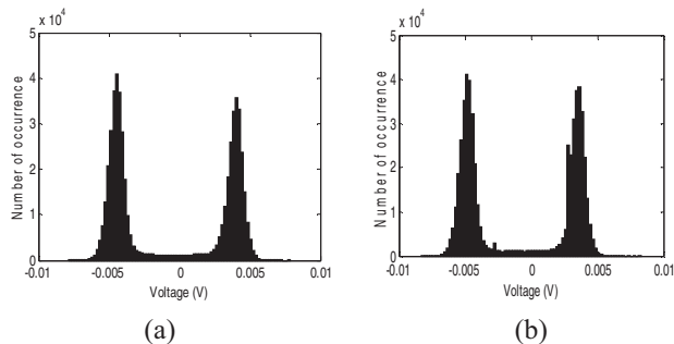
Figure A5. Received signal distribution for BPSK for a 50 mV p-p input signal: (a) without scintillation, and (b) with scintillation.
