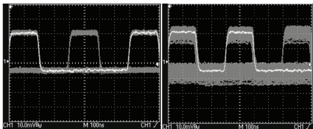
Figure 6. Eye diagram representations of OOK-RZ for a 100 mV p-p input signal; Received voltage is 10mV/div: (a) without turbulence, and (b) with turbulence
