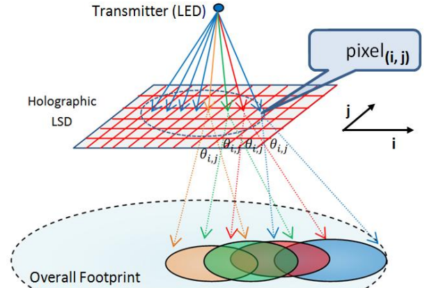
Fig. 4. Multiple beams profile after holographic LSD
