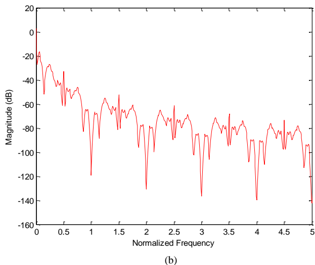
Figure 1. PSD of 8-CC-DPIM with 100% pulse duty cycle against the normalized frequency: (a) predicted, and (b) simulated
