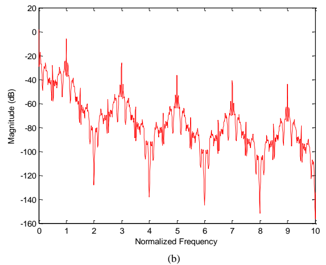
Figure 2. PSD of 8-CC-DPIM with 50% pulse duty cycle against the normalized frequency: (a) predicted, and (b) simulated
