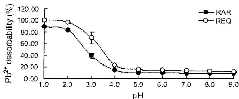
Figure 1.3 The desorption characteristics of lead as a function of pH (Yang et al. , 2006)
