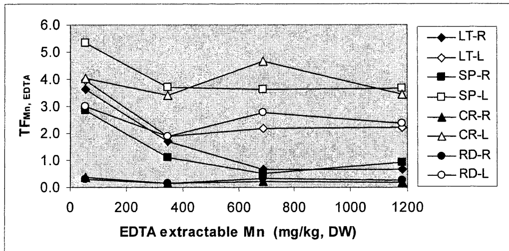
Figure 5.11 Relationship between the TF values of Mn (y) and EDTA extractable Mn in soils (x)
