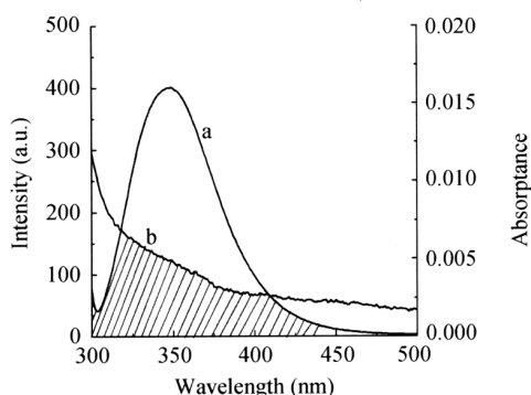
图4 相同浓度下( 5 \times 10^{-6} mol/L),BSA荧光图谱与胶毒素紫外—可见吸收谱的叠加 Fig. 4 The overlap of the fluorescence spectrum of BSA (a) and the absorbance spectrum of Gliotoxin (b) [C(BSA)=C(Gliotoxin)= 5 \times 10^{-6} mol/L]
