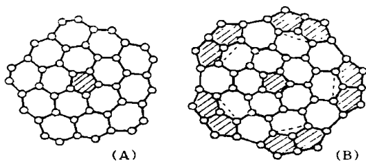
Fig. 1 Plane-shape molecule C 45 (A) (D 5h ) and C 60 (B) (D 5h )
