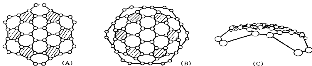
Fig. 2 Diagram of molecule C_{48}(D_{6h}) (A) and C_{60}(C_{6v}) (B) and its vertical view (C)
