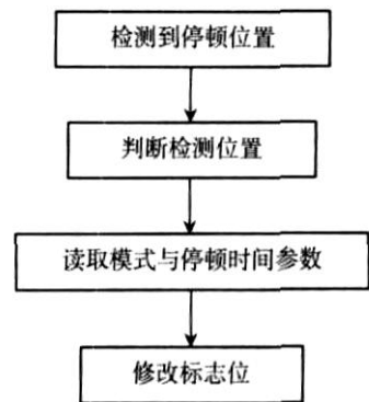
图 7 位置检测外部中断程序流程图 Fig.7 Flow chart of external interrupt program of position detection
