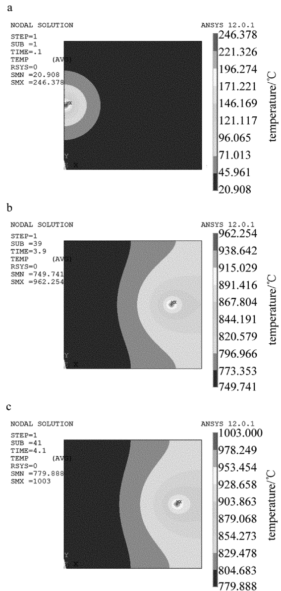
Fig. 7 Temperature field distribution at different time a—0.1s moment b—3.9s moment c—4.1s moment
