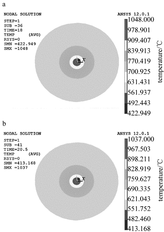
Fig. 6 Temperature field distribution under different reaction sources of gas flow
