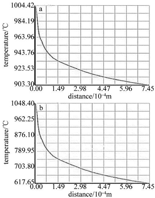
Fig. 5 Temperature along the node mapping a—copper substrate b—nickel substrate
