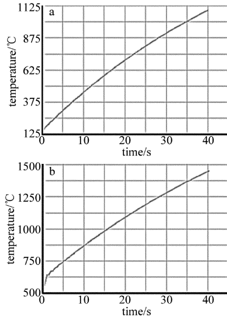
Fig. 4 Temperature change at the center spot a—copper substrate b—nickel substrate
