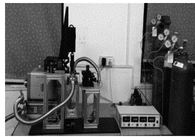
Fig. 1 Device of graphene fabrication with LCVD
