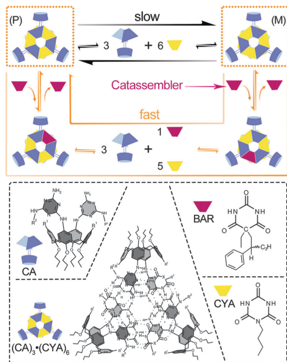
Fig. 2 Racemization of the enantiomers ( P ) and ( M ) under the disassembly–reassembly and catassembled processes. In the normal disassembly–reassembly racemization process, which is represented by the long black arrow, the ( P )- or ( M )-enantiomer of (CA)_3 \cdot (CYA)_6 first disassembles into the building blocks CA and CYA; then, the building blocks reassemble into the two enantiomers. In the catassembled racemization process represented by the long orange arrow, one of the CYA building blocks in the ( P )- or ( M )-enantiomer of (CA)_3 \cdot (CYA)_6 is first displaced by the chiral catassembler BAR and forms a ternary complex (CA)_3 \cdot (BAR) \cdot (CYA)_5 , which further changes into the corresponding ternary enantiomer through a disassembly–reassembly process. The BAR in the ternary enantiomer is finally displaced by CYA and forms the other enantiomer of (CA)_3 \cdot (CYA)_6 . The molecular structures of CYA, BAR, CA and enantiomer ( P ) are presented in the dashed box. Structural images adapted from ref. 62 (Copyright (2000), with permission from Nature Publishing Group).
