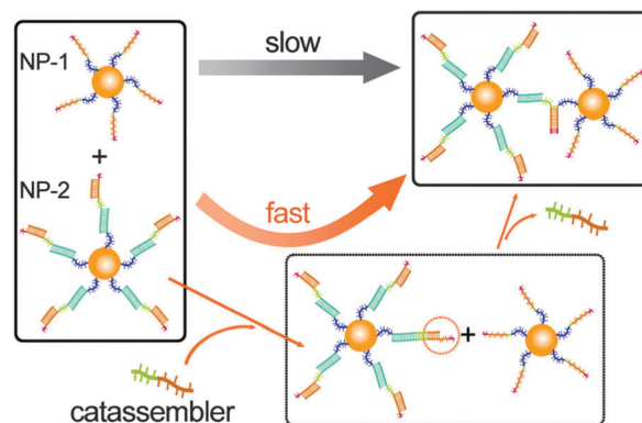
Fig. 5 Graphical representation of self-assembly and catassembler processes of DNA-modified Au NPs.
