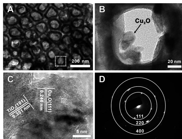
Fig. 2 (A) Low magnification TEM image of Cu 2 O/TiO 2 NTAs prepared by the ultrasonication-assisted S-CBD for 4 min (top view). (B) Close-up of the selected area marked in (A). (C) The high resolution TEM image of Cu 2 O/TiO 2 NTAs. (D) The selected area electron diffraction (SAED) pattern of Cu 2 O taken from the nanoparticles in (C).
