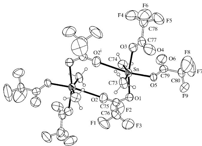
Figure 1 ORTEP II (Johnson, 1976) plot of the [\text{Sn}(\text{CH}_3)_2(\text{O}_2\text{CCF}_3)_3]_2^{2-} dianion, with displacement ellipsoids drawn at the 50% probability level. Only one set of F atoms of the disordered trifluoromethyl group is shown. H atoms are drawn as spheres of arbitrary radii. [Symmetry code: (i) 1 - x, 1 - y, 1 - z .]
