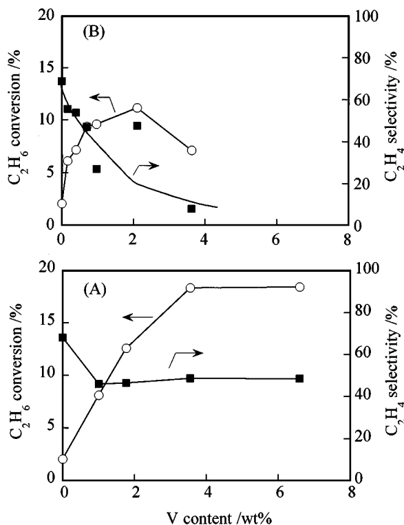
FIG. 7. Results for catalytic oxidation of C 2 H 6 over V-MCM-41 by TIE (A) and DHT (B) methods. (○) C 2 H 6 conversion, (■) C 2 H 4 selectivity. Conditions: W = 0.2 g, T = 550^\circ\text{C} , F = 50 ml/min, P(\text{C}_2\text{H}_6) = 12.2 kPa, P(\text{O}_2) = 6.1 kPa.
