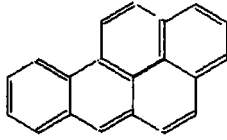
图 1 苯并 [ a ] 芘 ( BaP ) Fig 1 Benzo ( a ) pyrene ( BaP )
