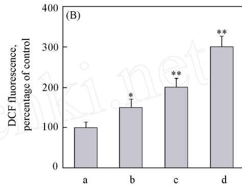
Fig 2 Fluorescence microscopy (A 1 —A 4 ) with DCF staining (B)
