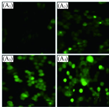
Fig 2 Fluorescence microscopy (A 1 —A 4 ) with DCF staining (B)
