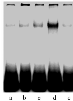
Fig 4 Effects of MWCNTs on NF- \beta activation in A549 cells assessed by EMSA
