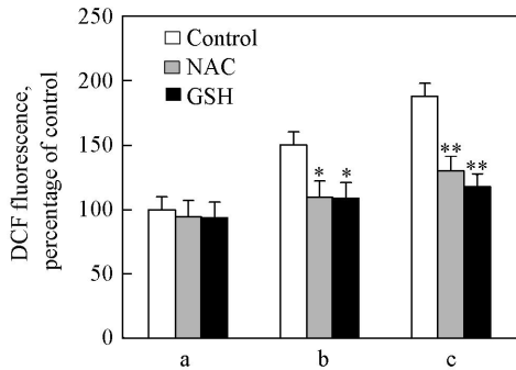
Fig 3 Effects of NAC and GSH on MWCNTs-induced ROS generation in A549 cells
