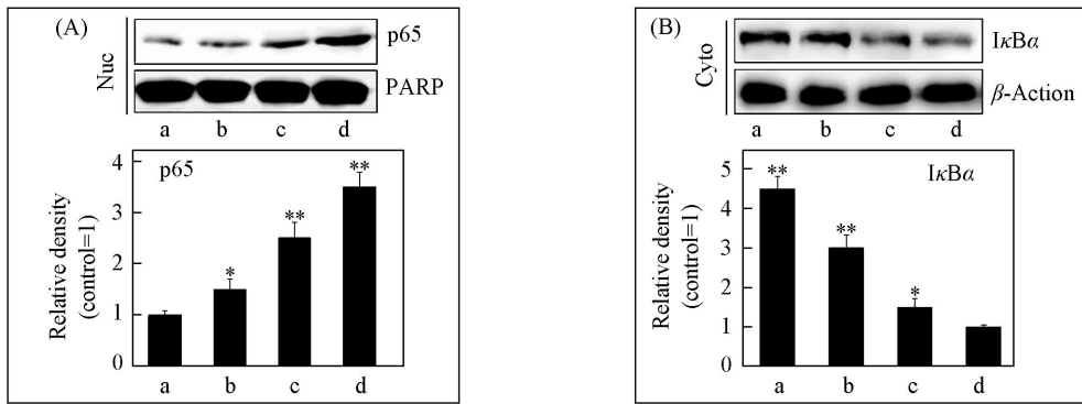
Fig 5 Effects of MWCNTs on the levels of nuclear p65 (A) and cytoplasmic I \kappa B (B) determined by Western blotting
