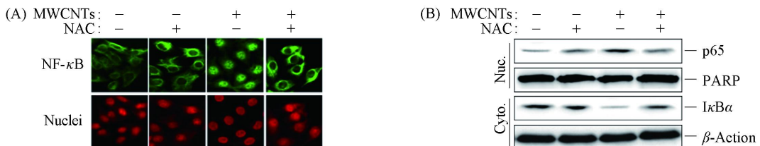
Fig 7 Effects of NAC on translocation of p65 into the nucleus examined by immunofluorescence confocal microscopy (A) and on the levels of nuclear p65 and cytoplasmic I \kappa B determined by Western blotting (B)
