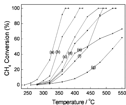
Fig. 1 Ignition curves of methane combustion over Pd-Zr/HZSM-5 (a), Pd/HZSM-5 (b), Pd-La/HZSM-5 (c), Pd-Al/HZSM-5 (d), Pd-Y/HZSM-5 (e), Pd/ \gamma\text{-Al}_2\text{O}_3 (f), and Pd/ \text{SiO}_2 (g). Feed composition: \text{CH}_4 (2%), \text{N}_2 (90%), \text{O}_2 (8%); \text{GHSV} = 48000 \text{ h}^{-1} .
