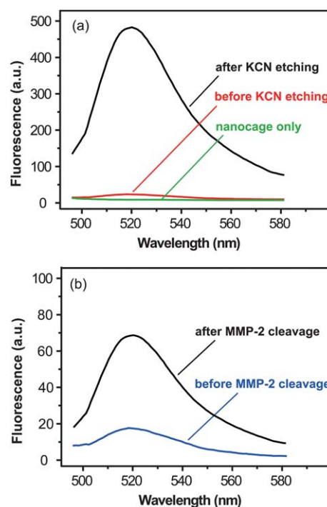
Fig. 2 (a) Fluorescence spectra of FITC-GKGPLGVRC-cage770 before and after KCN etching; (b) fluorescence spectra of FITC-GKGPLGVRC-cage770 before and after incubation with 1 U (72 ng mL -1 ) MMP-2 at 37 °C for 3 h.
