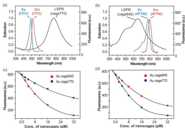
Fig. 5 Spectroscopic characterization of the Au nanocages and dyes: (a) excitation and emission spectra of FITC and extinction spectrum of Au nanocages with LSPR peaked at 770 nm (cage770); and (b) excitation and emission spectra of Alexa Fluor 790 (AF790) and extinction spectrum of Au nanocages with LSPR peaked at 645 nm (cage645). (c, d) Plots of the fluorescence intensity as a function of nanocage concentration where a specific amount of the dye was mixed with the Au nanocages of different concentrations in aqueous solutions: (c) FITC at a final concentration of 10^{-7} M and (d) AF790 at a final concentration of 10^{-6} M.
