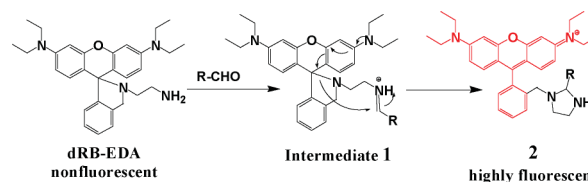
Scheme 1 Detection of aldehydes with dRB-EDA via tandem imine formation and intramolecular cyclization.
