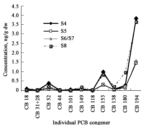
Fig. 2 Distribution of individual PCBs congeners in different samples
