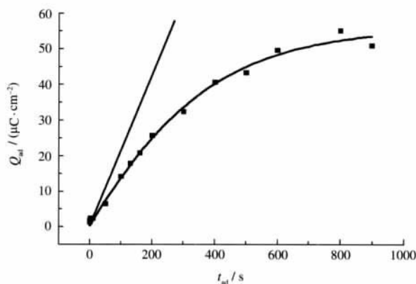
图6 E_{ad}=0.10 \text{ V} 时 Pt(111)-II 电极 Q_{ad} 随 t_{ad} 的变化 Fig.6 Variation of Q_{ad} with t_{ad} for Pt(111)-II when E_{ad}=0.10 \text{ V}
