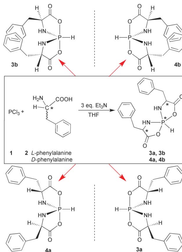
Scheme 1 Structures of spirophosphoranes 3a , 3b , 4a and 4b .
