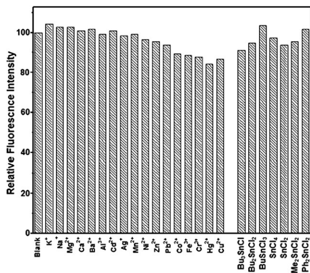
Fig. 4 The influence of coexistence of other metal species on the fluorescence response of 2 to 20 equiv. of \text{BuSn}(\text{OH})_2\text{Cl} in \text{H}_2\text{O} –EtOH (90 : 10, v/v). 2 : 1.0 \times 10^{-6} M; pH: 7.4, buffered by 0.01 M Tris-HCl; \lambda_{\text{ex}}/\lambda_{\text{em}} : 403/474 nm. \text{K}^+ , \text{Na}^+ , \text{Mg}^{2+} , \text{Ca}^{2+} , \text{Ba}^{2+} , \text{Al}^{3+} : 1000 equiv.; \text{Cd}^{2+} , \text{Ag}^+ , \text{Mn}^{2+} , \text{Ni}^{2+} , \text{Zn}^{2+} , \text{Pb}^{2+} , \text{Co}^{2+} , \text{Fe}^{3+} , \text{Cr}^{3+} : 100 equiv.; \text{Hg}^{2+} , \text{Cu}^{2+} , \text{Bu}_3\text{SnCl} , \text{Bu}_2\text{SnCl}_2 , \text{BuSnCl}_3 , \text{SnCl}_4 , \text{SnCl}_2 , \text{Me}_2\text{SnCl}_2 , \text{Ph}_2\text{SnCl}_2 : 20 equiv.
