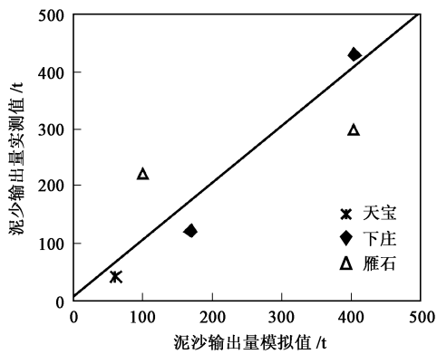
图3 九龙江典型小流域泥沙输出模拟值与实测值拟合图 Fig.3 Comparison of simulated and observed sediment for model calibration in typical sub-watersheds
