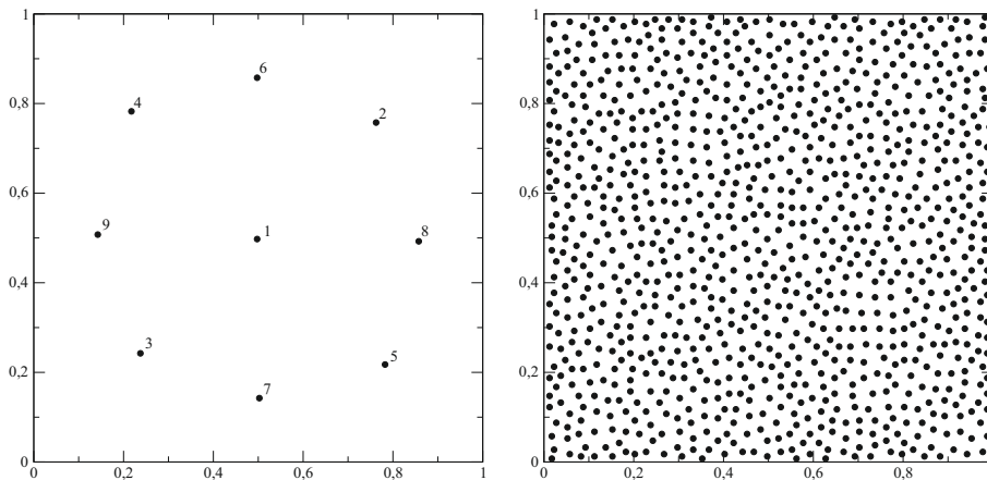
FIGURE 3. Short-term location for the case of a uniform density on a unit square of (left) the first 9 points (right) 1000 points.
