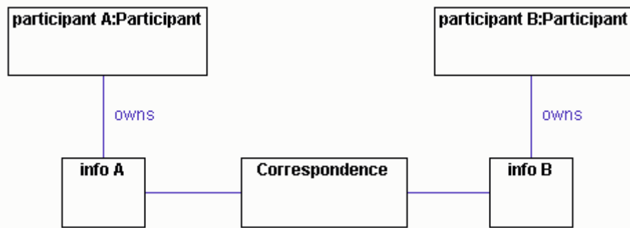
Figure 3. Object diagram showing the Correspondence pattern structure
