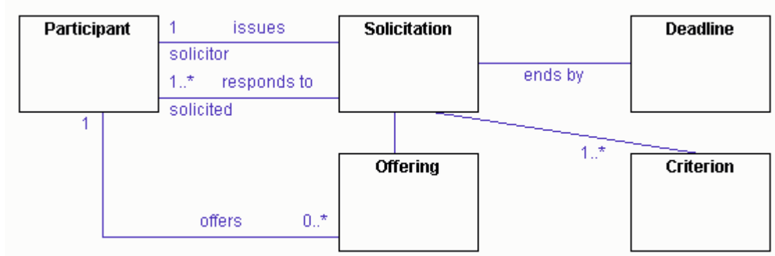
Figure 5. Class diagram showing the Solicitation pattern structure
