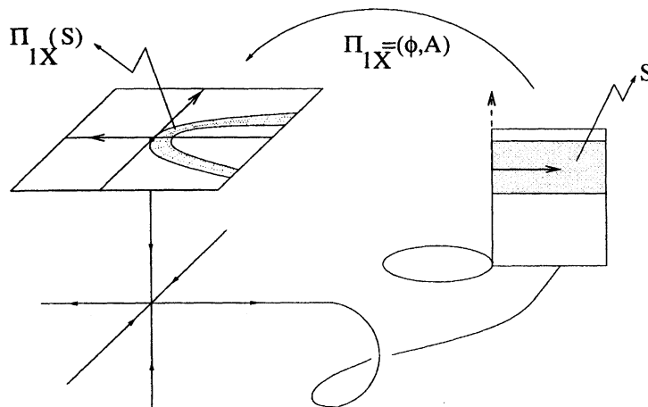
The case \partial_{yy}\phi(0,1,X) > 0 and \partial_y A(0,1,X) > 0
