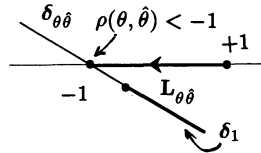
Figure 4.d : \theta' = \hat{\theta} .
