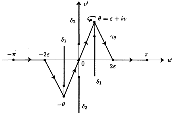
Figure 3.c : \theta = \epsilon + iv .
