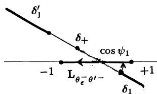
Figure 10.b : \theta' = \theta'^- .
