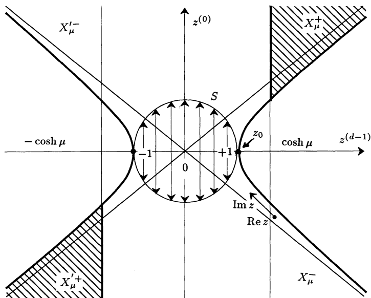
Figure 8. The hyperboloid X and the regions X_\mu^+, X'^+_\mu (in hatchings) and X_\mu^-, X'^-_\mu . A typical point \text{Re } z + i\text{Im } z of X^{(c)} and the sphere S are illustrated via the “arrow representation” of complex points.
