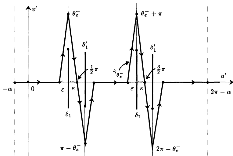
Figure 9.c : \theta = \theta_\epsilon^- .
