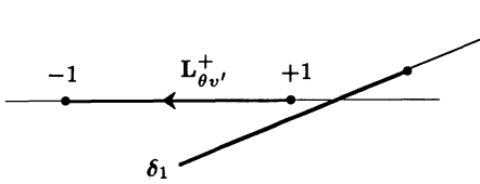
Figure 4.e : \theta = \varepsilon + iv, \theta' \in [0, \theta] .
