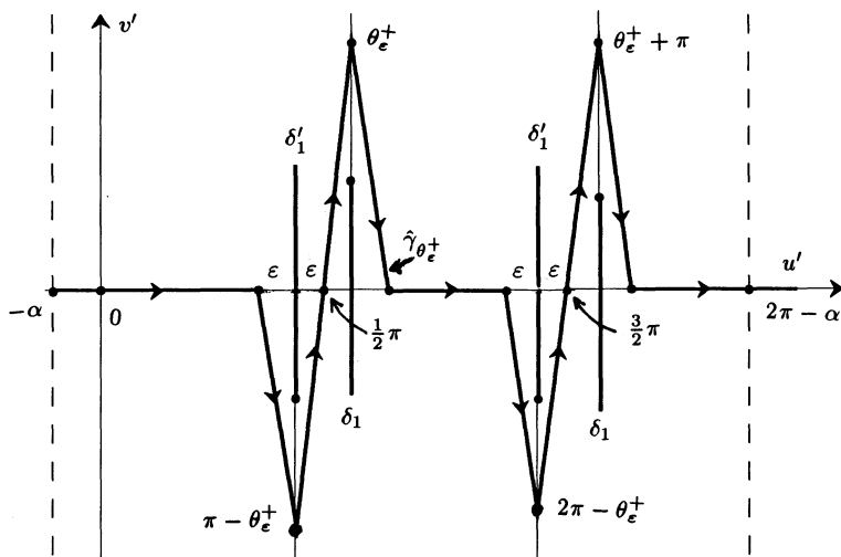
Figure 9.b : \theta = \theta_\epsilon^+ .
