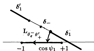
Figure 10.a : \theta' = \theta'^+ .
