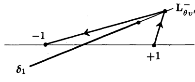
Figure 4.f : \theta = \varepsilon + iv, \theta' \in [\theta, 2\varepsilon] .
