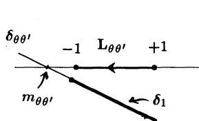
Figure 4.a : \theta' \in [\pi - u, \pi] .
