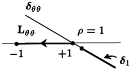
Figure 4.c : \theta' = \theta .
