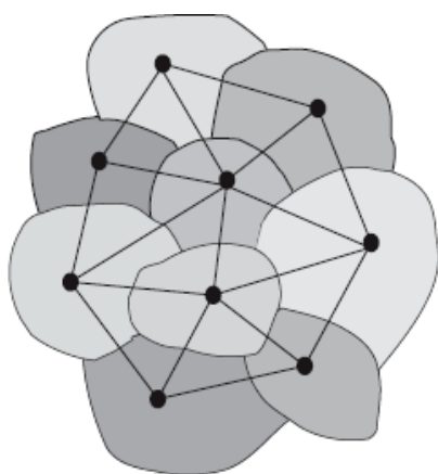
Figure 7.1: Quanta of volume (grey blobs). Adjacent chunks are separated by a surface \mathcal{S} of quantised area. The corresponding spin network graph is overlaid. Each link “cuts” one quantised surface \mathcal{S} .
