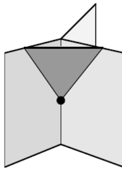
Figure 7.8: Vertex of a spin foam. (Rovelli, 2004, p. 325).
