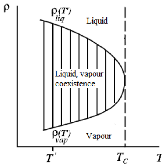
Figure 4.2: Coexistence curve for a fluid. (Adapted from Batterman, 2011, p. 1036)
