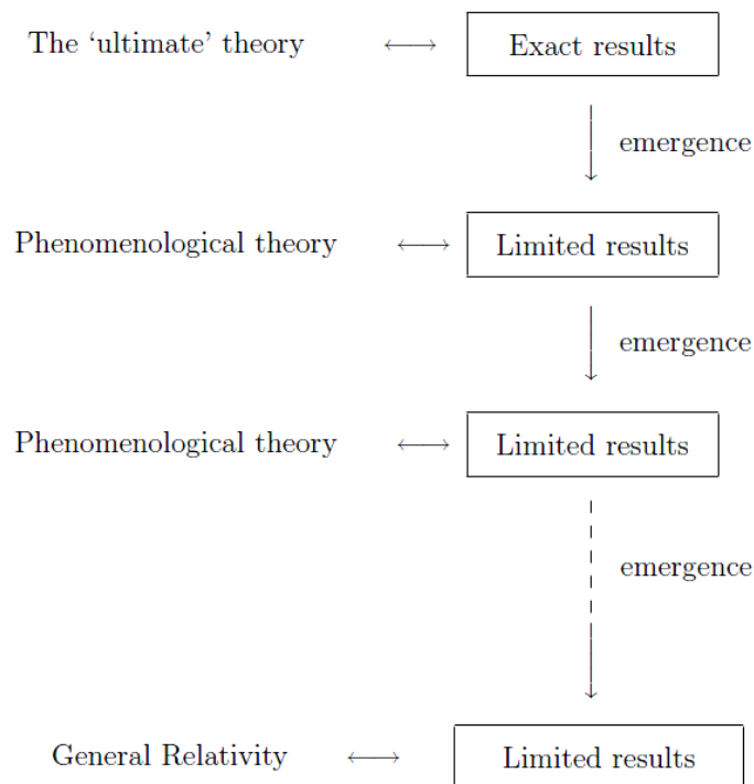
Figure 2.1: Tower of emergent theories. (Adapted from Butterfield and Isham, 2001, p. 79)
