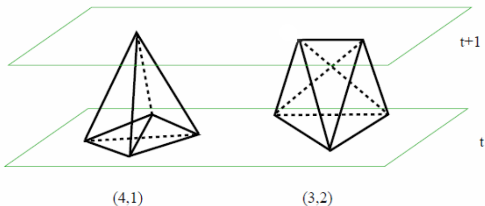
Figure 6.3: The two fundamental building blocks of CDT. The four-simplex (4,1) has four of its vertices at time t and one at time t + 1 , and analogously for the (3,2) type of simplex. (From Ambjørn et al. (2009, p. 347)).
