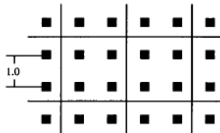
(b) Rescaling : the lengths are shrunk in order to recover the original lattice spacing of 1.
