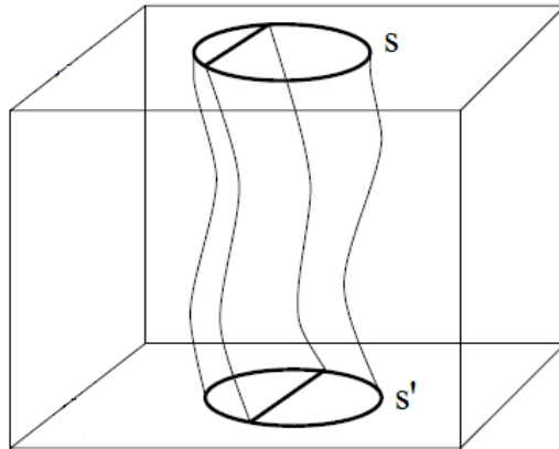
Figure 7.7: A simple spinfoam: the worldsheet of a spin network (“colouring” of the faces and edges not indicated). (Adapted from Rovelli, 2004, p. 325).
