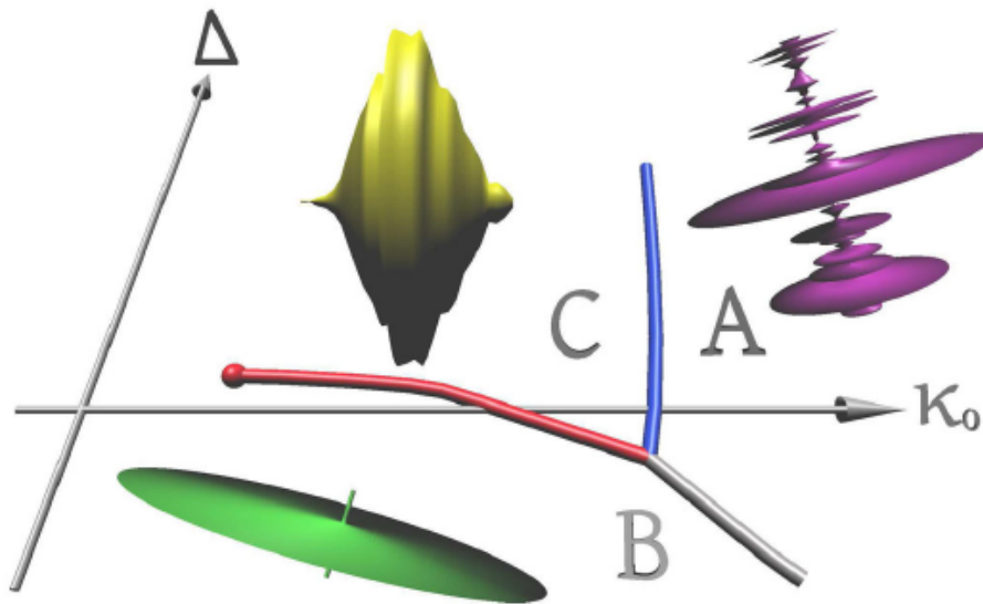
Figure 6.5: Visualisation of the CDT phase diagram, based on actual measurements, illustrating the distinct volume profiles characterising the three observed phases A, B and C. (From Ambjørn, Jordan, et al., 2012, p. 124044-3).
