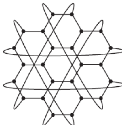
Figure 6.7: Low-energy (post-geometrogenesis) phase of quantum graphity. (Markopoulou, 2008).
