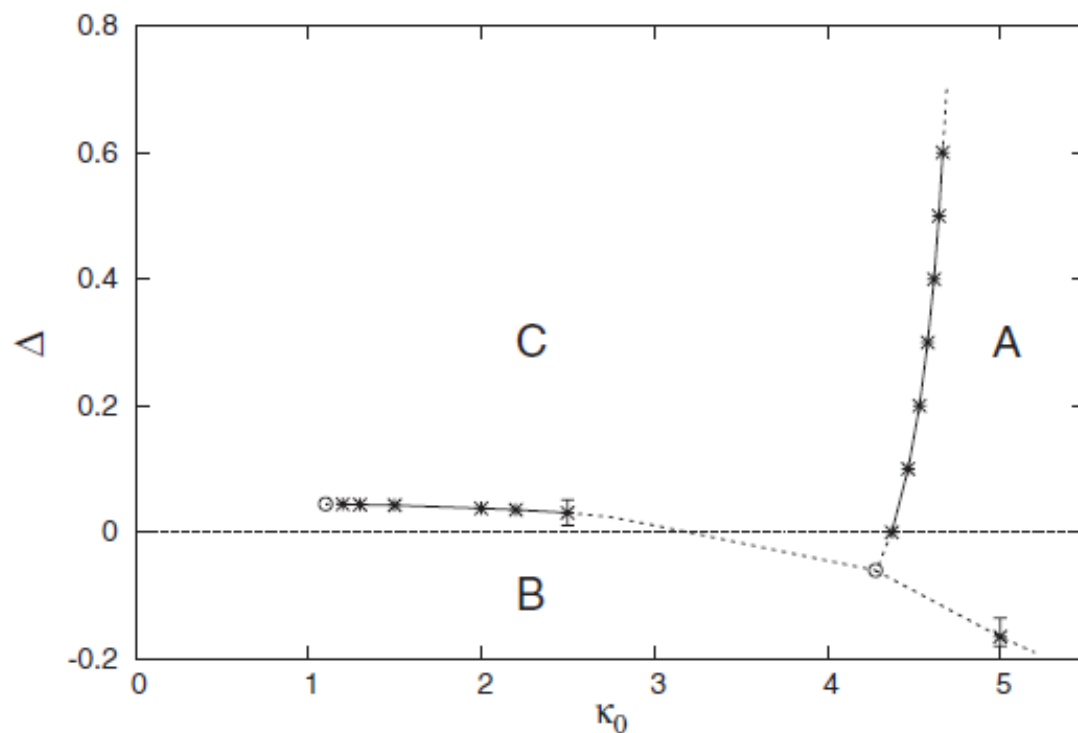
Figure 6.4: Phase diagram of CDT. Crosses represent actual measurements, dashed lines are extrapolations. (From Ambjørn, Jordan, et al., 2012, p. 124044-3).
