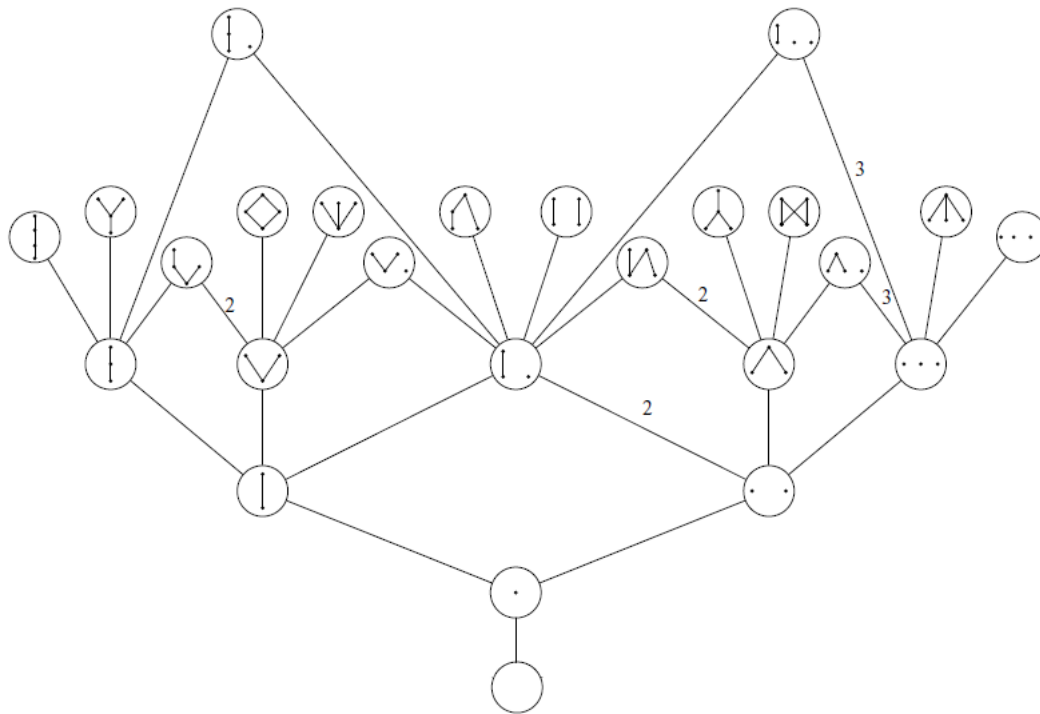
Figure 6.2: Hasse diagram depicting the partially ordered set of finite causets (only causets up to size 4 are shown). The elements of this set are the finite causets. The numbers on some links indicate the number different possible ways in which new elements can be added, due to automorphisms of the “parent” causet. (Adapted from Henson (2009)).
