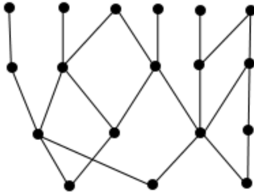
Figure 6.1: Hasse diagram of a causal set.
