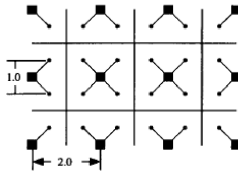
(a) Block spin formation : Ising model with lattice spacing of 1 (small round dots). The spins are grouped into blocks of 4 and replaced by block spins (large square dots), the block spins having a lattice spacing of 2.
