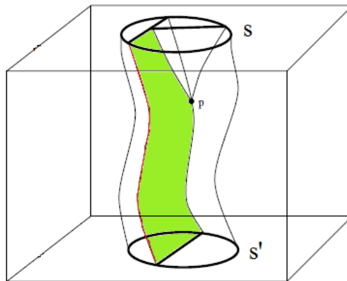
Figure 7.9: Spinfoam with one vertex. One face has been tinted green, and one edge is shown in red. (Adapted from Rovelli, 2004, p. 326).
