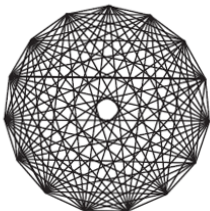
Figure 6.6: High-energy (pre-geometric) phase of quantum graphity. (Markopoulou, 2008).
