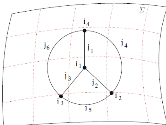
Figure 7.4: A spin network embedded on the spatial hypersurface \Sigma (adapted from Nicolai & Peeters (2007, p. 156)).
