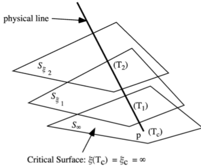
Figure 4.3: The “physical line” of a system, parametrised by temperature, intersecting several surfaces of constant correlation length in parameter space. Where \xi(T_1) = \xi_1 , \xi(T_2) = \xi_2 , with \xi_1 > \xi_2 , and \xi(T_c) = \infty
