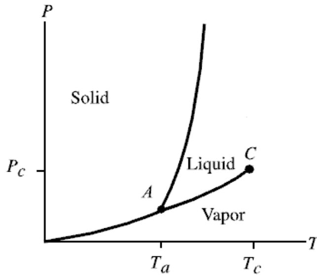
Figure 4.1: Temperature-pressure phase diagram for a fluid. (Adapted from Batterman, 2011, p. 1035)
