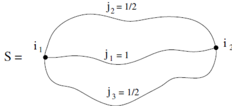
Figure 7.3: A simple spin network with colouring. Labels i_n indicate the quantised volume of the corresponding node, and j_l give the quantised area represented by the corresponding link. (Rovelli, 2004, p. 19).
