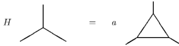
Figure 7.5: Scheme of the action of H on a node of a spin network. (Rovelli, 2004, p. 25).
