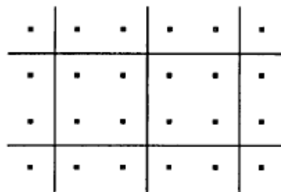
(c) Renormalisation : interaction parameters are adjusted in order to preserve the large-scale properties of the original lattice.
