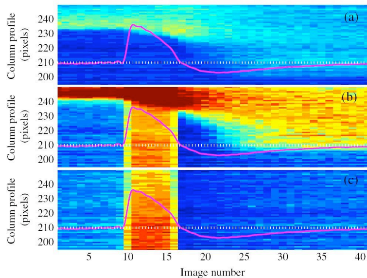
Figure 5.4: LRR heartbeat instability: current amplitude superimposed on column profile for (a) only dust cloud; (b) dust cloud and plasma glow; (c) plasma glow only. Parts (a), (b) and (c) are in false colours from dark blue to red
