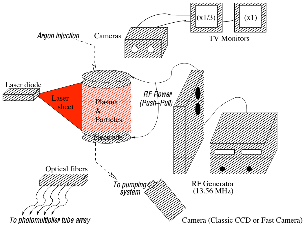
Figure 3.4: Principle schematic of optical diagnostics
