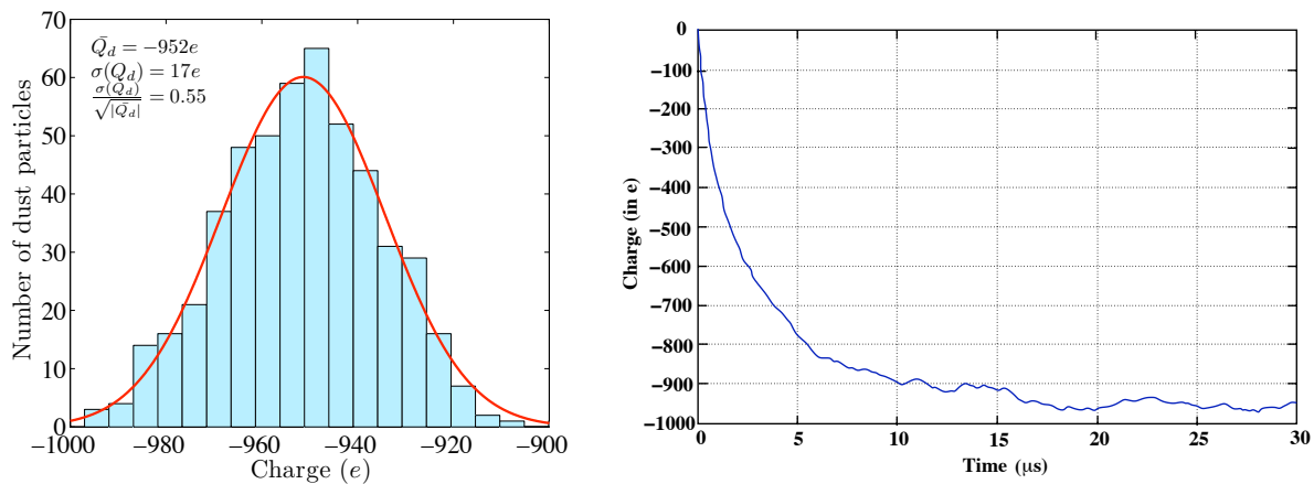
Figure 2.2: Calculation of dust particle charges using a Fokker-Planck algorithm [93] for 190 nm radius particles in a plasma with T_e = 3 \text{ eV} , T_i = 0.03 \text{ eV} and n = n_e = n_i = 5 \cdot 10^9 \text{ cm}^{-3} . Left: Dust particle charge distribution for 500 iterations. Right: Dust particle charge evolution when immersed in the plasma
