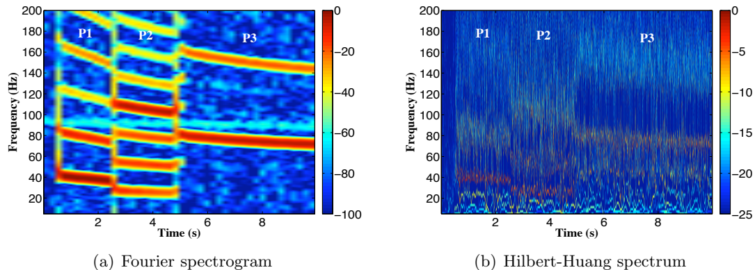
Figure 4.17: Fourier spectrogram and Hilbert-Huang spectrum during the three first phases of DPGI. In this figure t = 0 does not correspond to the plasma ignition but corresponds to a time close to the DPGI beginning.
