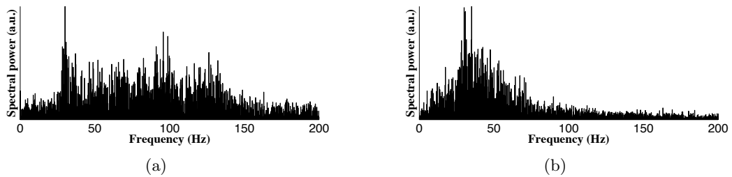
Figure 4.23: Fourier spectrum of the first chaotic regime. (a) on current signal (b) on central optical fibre signal
