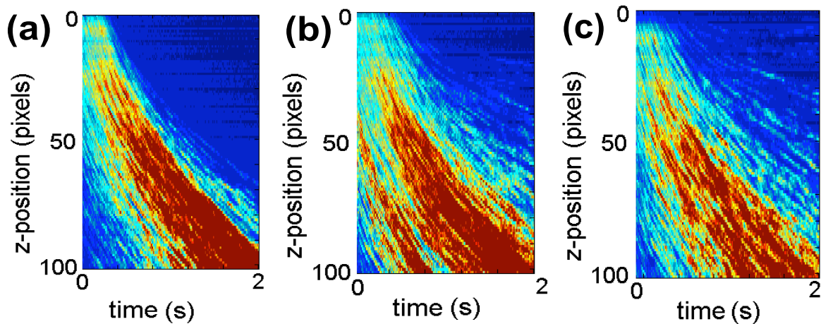
Figure 6.8: Line profile of a high speed video imaging during the fall of the dust particle cloud in discharge afterglow at P = 1.6 mbar (in false colour from blue to red). (a) No bias on the lower electrode. (b) -10V bias on the powered electrode. (c) +10 V bias on the power electrode
