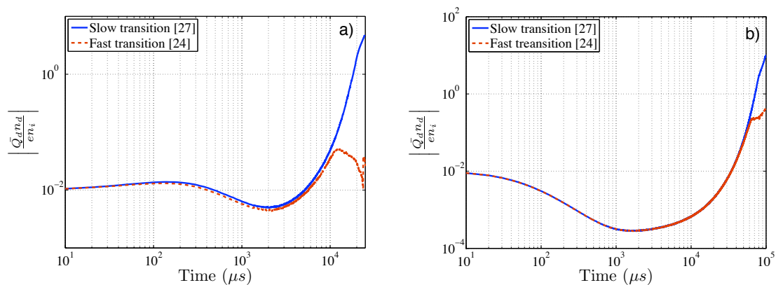
Figure 6.23: Evolution of |\bar{Q}_d n_d / e n_i| . a) P = 0.4 \text{ mbar} . b) P = 1.2 \text{ mbar}
