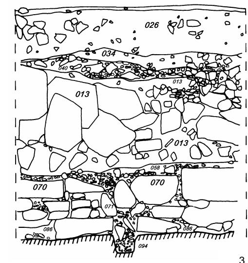
North Section
