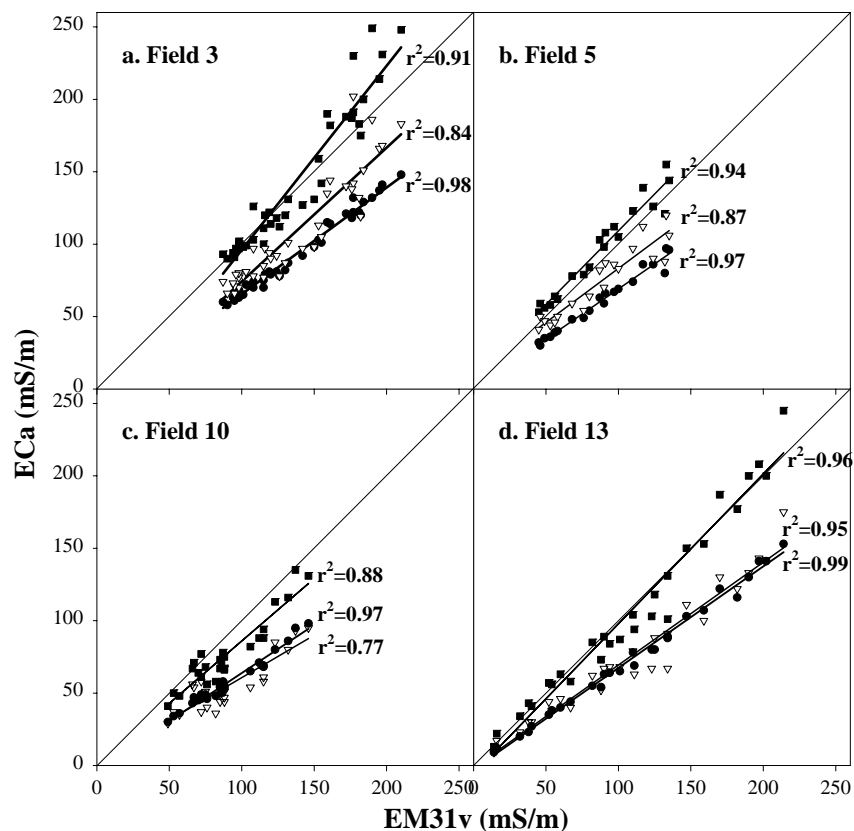
Figure 12. EM31v values plotted against EM31H (◻), EM38v (⊠) and EM38H (◻) for a) field 3, b) field 5, c) field 10 and d) field 13.
