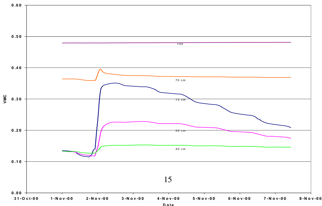
Fig. 1 3a. VWC increase after a rain event of 37mm in a wheat plot - site 2, 2000
