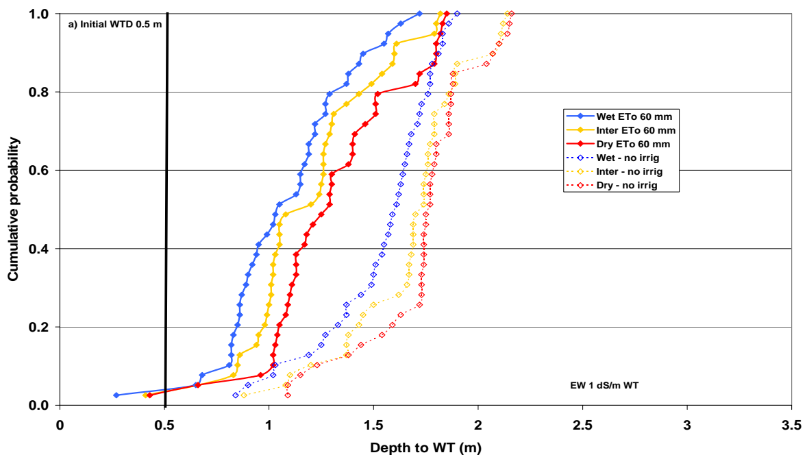
Figs 22a-c. Effect of irrigation frequency on final depth to watertable for early wheat
