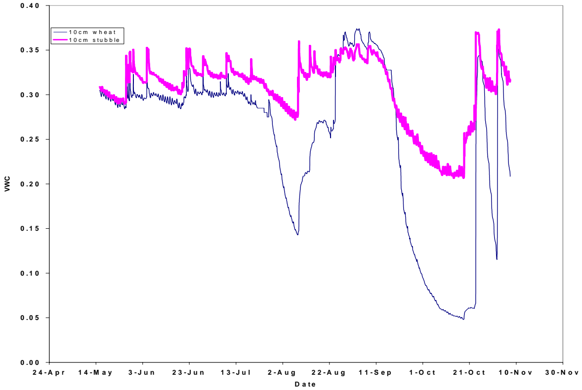
Fig. 13b. VWC @ 10cm for wheat and stubble
