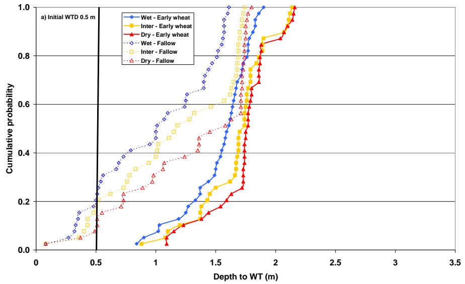
Figs 18a-c. Effect of initial SWC and WTD on final watertable depth for early wheat compared with fallow landuse (initial watertable salinity 1 dS/m, no irrigation)
