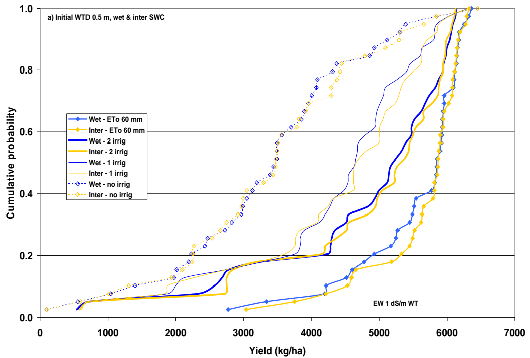
Figs 21a-c Effect of irrigation at key growth stages on yield of early wheat, 1 dS/m initial watertable salinity
