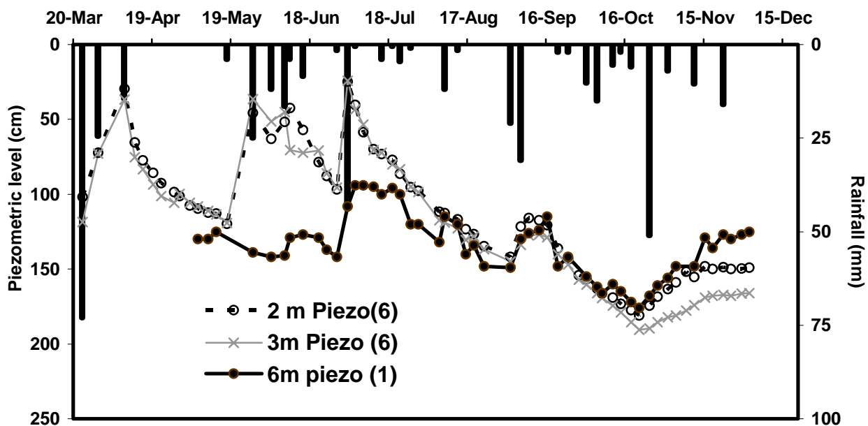
Fig. 6. Piezometer pressure levels in wheat plots (2 m, 3 m) and adjacent to experiment (6 m) at Site 1 in 1999
