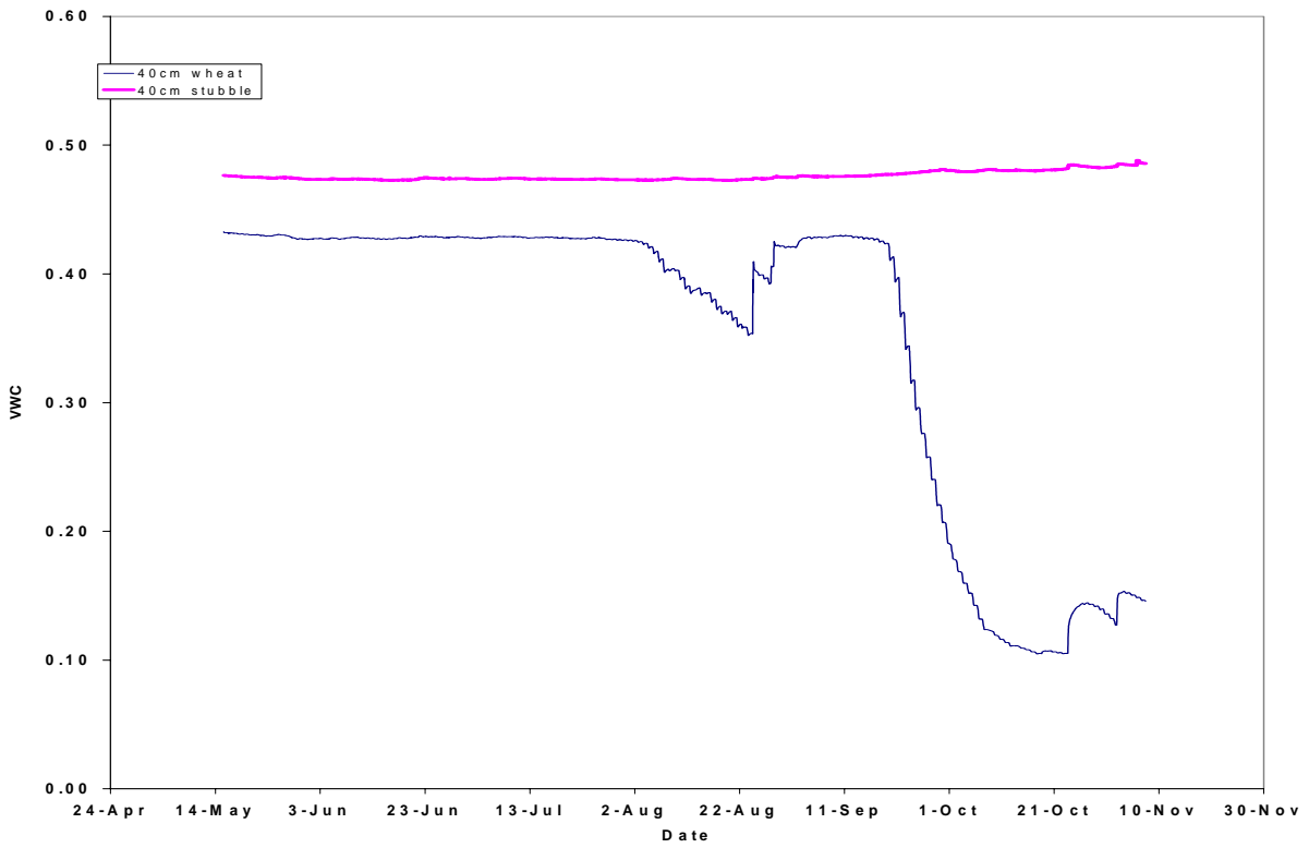
Fig. 13c. VWC @ 40cm for wheat and stubble
