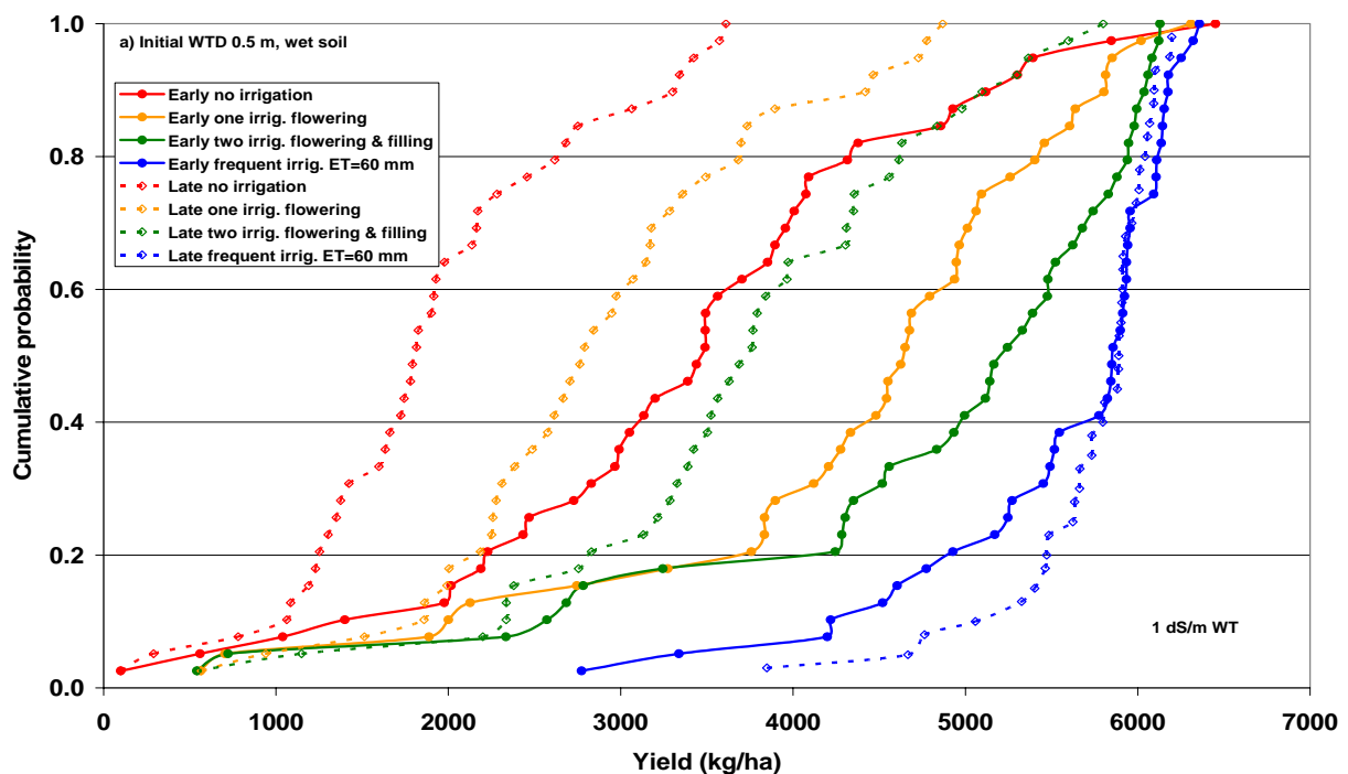
Fig. 24a. Yield of early and late wheat as affected by irrigation frequency and initial WTD and SWC (1 dS/m watertable)
