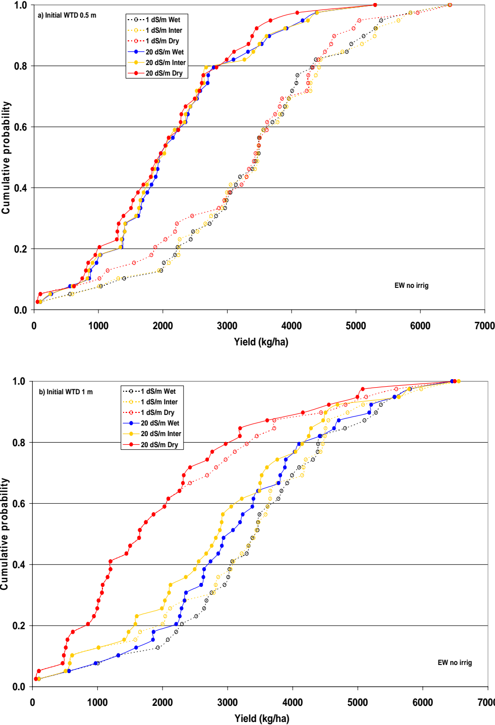
Figs 20a,b. Yield of early wheat as affected by initial watertable salinity
