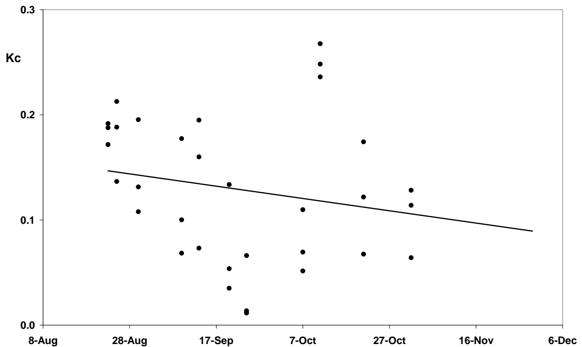
Fig. 8. Fallow “crop” factor ( K_c = \text{soil evaporation}/ET_o ) determined in microlysimeters at Site 1 in 1999
