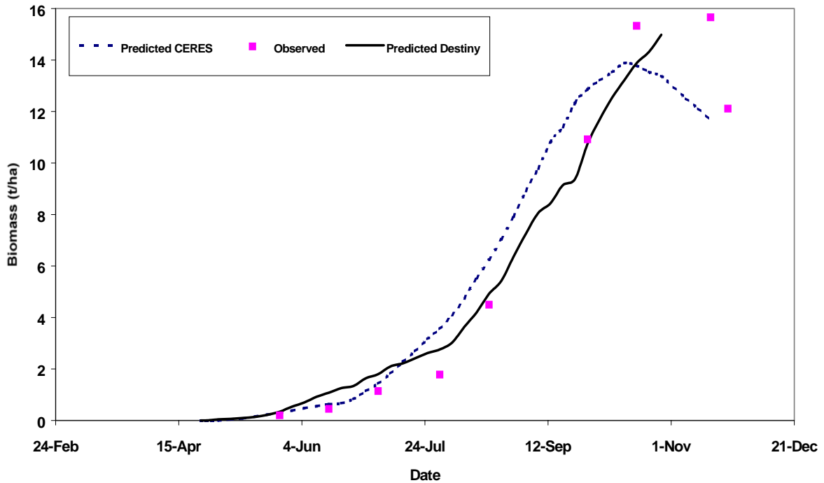
Fig. 16. Observed and simulated above ground biomass for early wheat in 1998, independent data set
