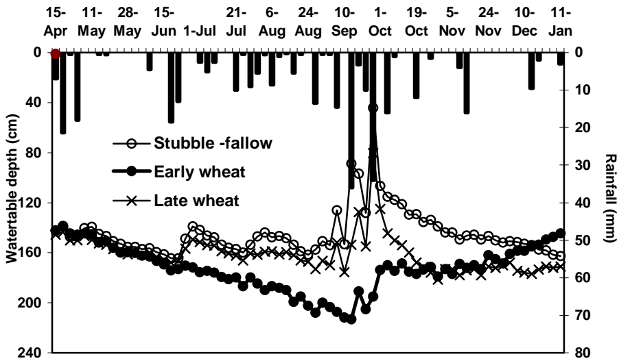
Fig. 1. Effect of sowing wheat after rice on depth to watertable - Site 1, 1998
