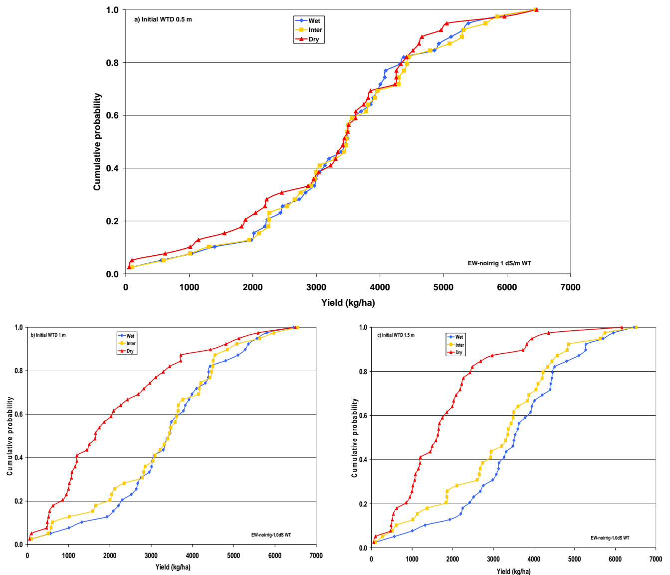
Figs 19a-c. Yield of early wheat as affected by initial SWC and WTD for 1 dS/m watertable, no irrigation
