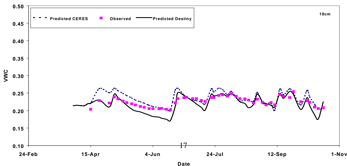
Fig. 14. Observed and simulated soil volumetric water content at 10 cm for early wheat in 1998, independent data set
