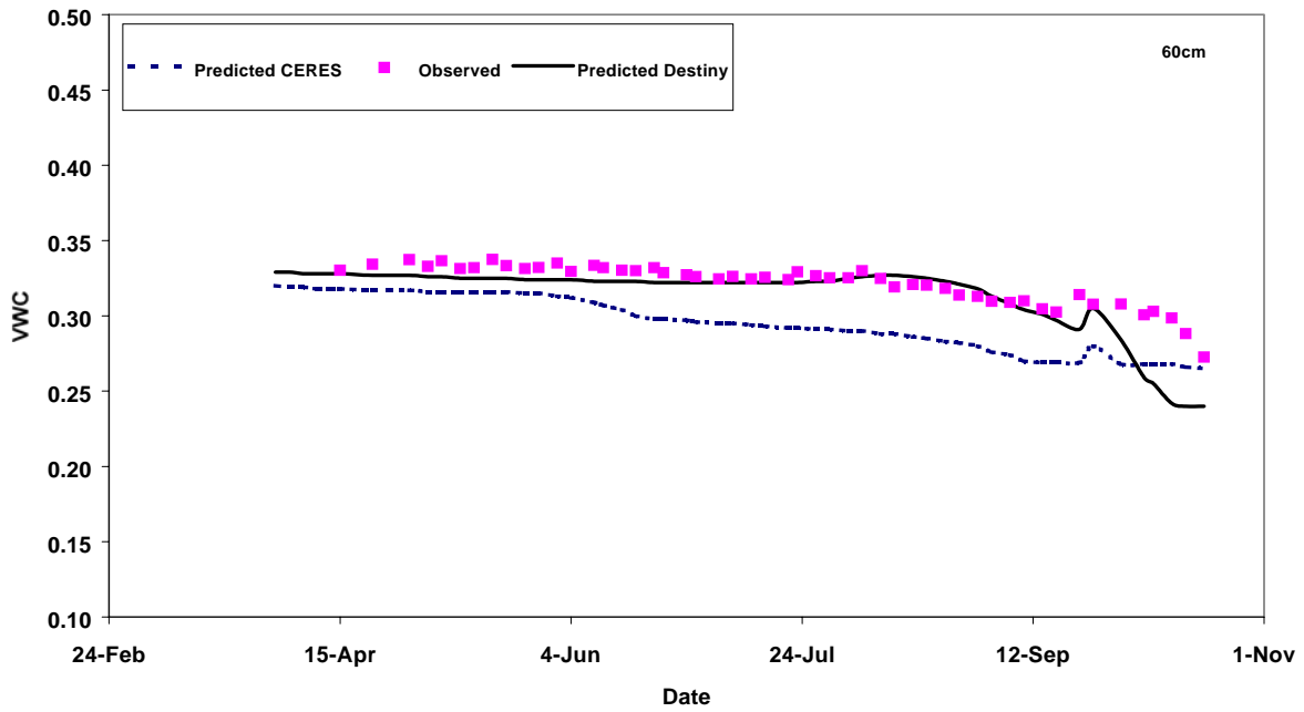
Fig. 15. Observed and simulated soil volumetric water content at 60 cm for early wheat in 1998, independent data set
