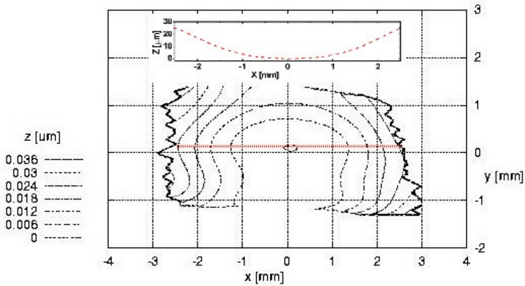
Fig.1 Surface curvature of 1μm thick Al 0.1 Ga 0.9 N layer on 60μm bulk GaN substrate.
