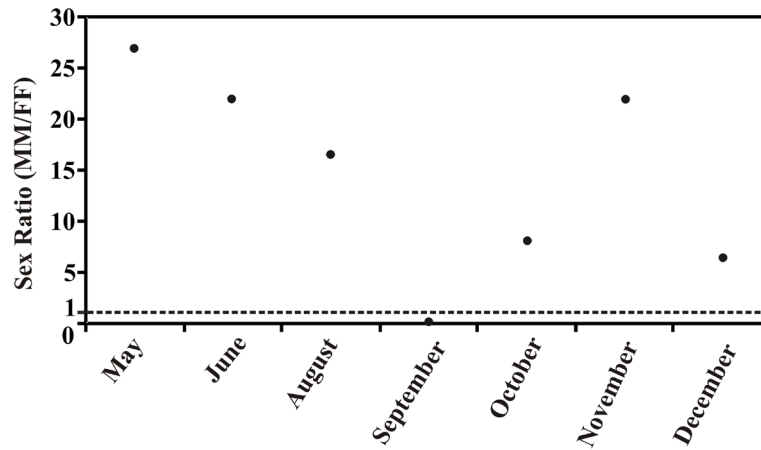
Figure 6. Monthly distribution of the sex ratio of C. aestuarii .
