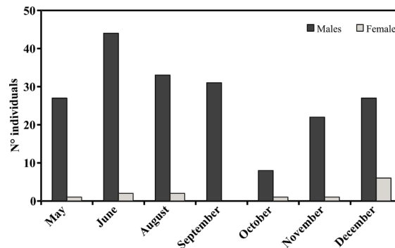
Figure 3. Monthly distribution of males and females.
