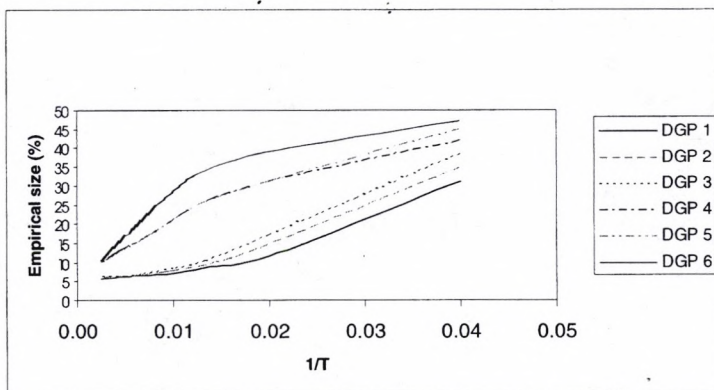
Figure 2: Rate of convergence (vs T^{-1} ) of the Wald test for \beta_2 .
