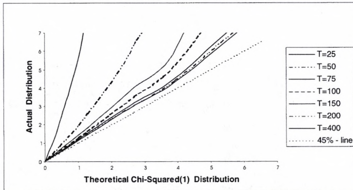
Figure 3: QQ-plot for DGP_3 : Wald test for \beta_2 .
