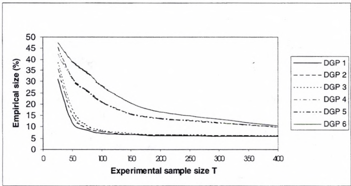
Figure 1: Simulated actual size of the Wald test for \beta_2 .
