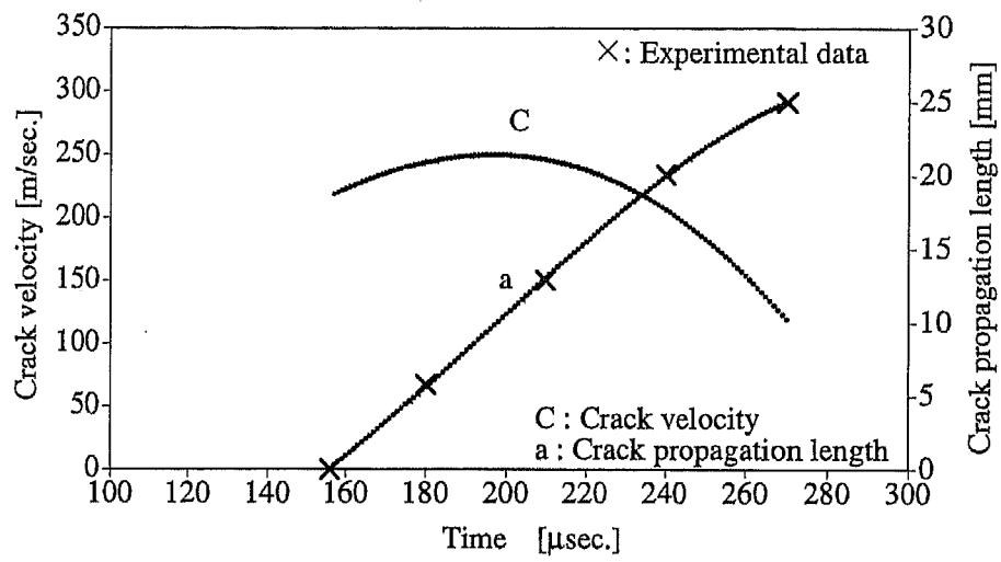
Fig.5 Crack propagation history ( e=0.0 )
