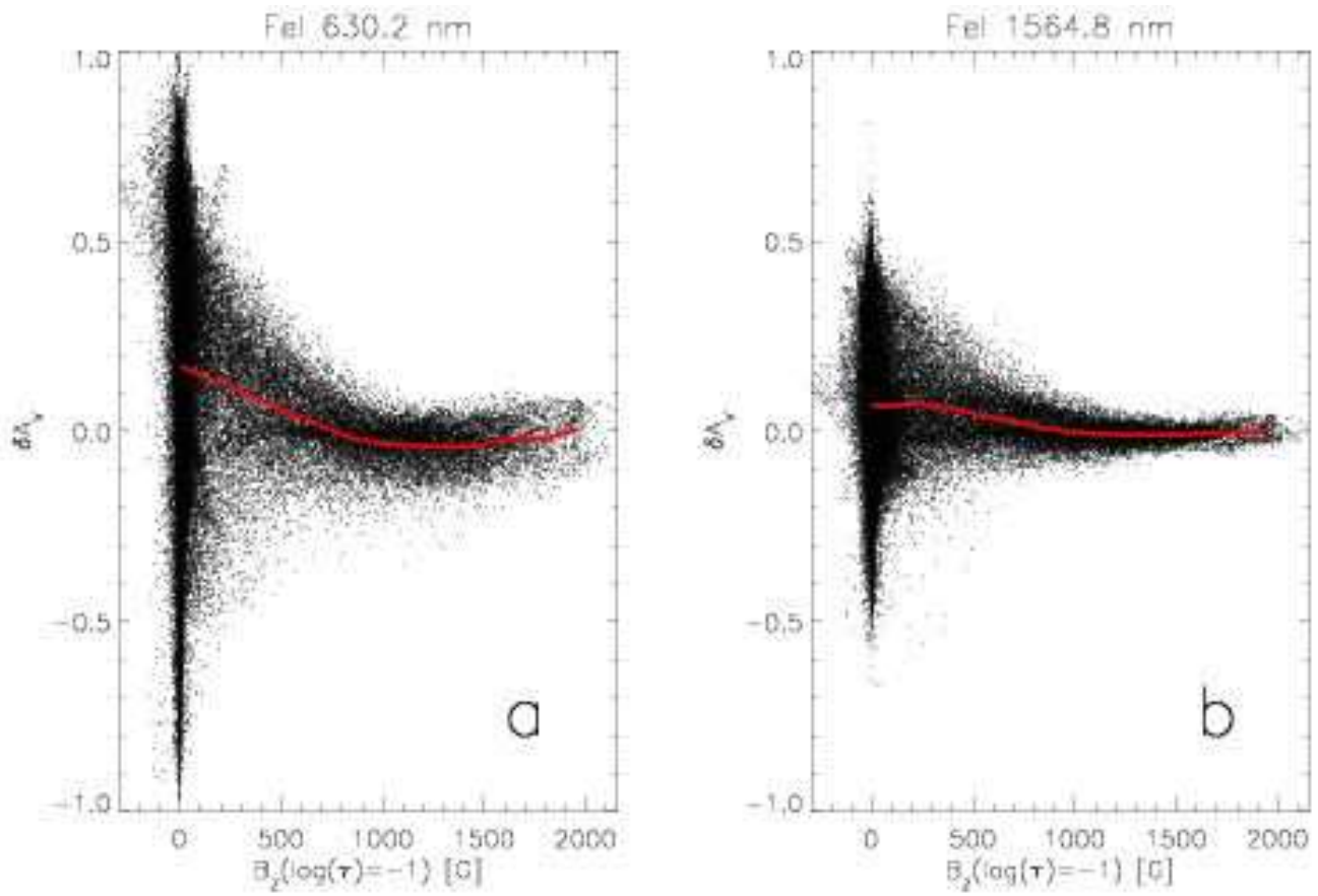
Fig. 15. Scatter plots of the Stokes- V area asymmetry versus the vertical (line-of-sight) component of the magnetic field at \tau_{500} = 0.1 a : Fe I 630.2 nm, b : Fe I 1564.8 nm. The lines show binned averages.
