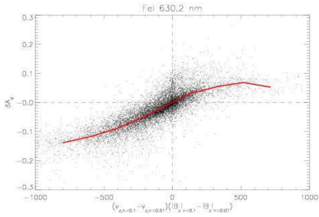
Fig. 19. Scatter plot of the Stokes- V area asymmetry for the 630.2 nm line versus a quantity representing the gradients of the line-of-sight magnetic field and velocity within the height range of line formation. The sign of the bin-averaged \delta A_V (indicated by the line) is in agreement with the relation given in Eq. (8).
