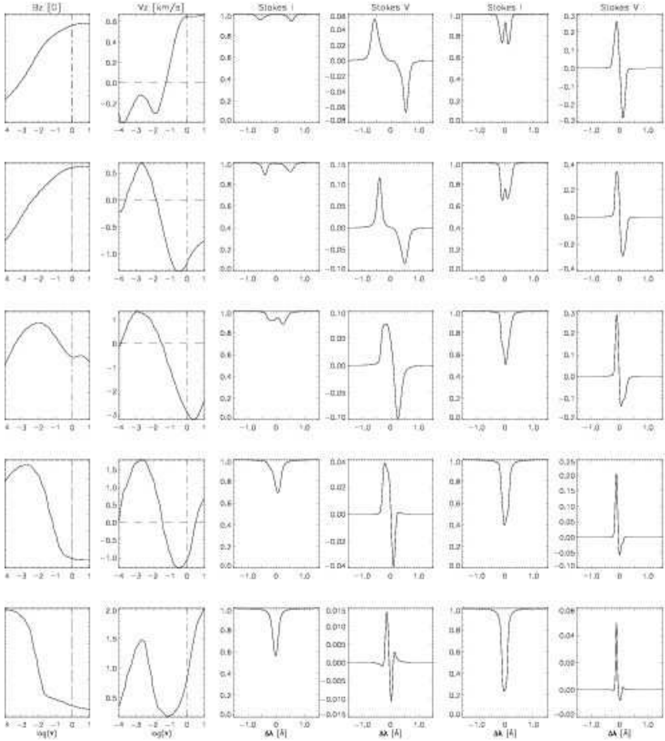
Fig. 11. Stokes- I and Stokes- V profiles for the 1564.8 nm line (third and fourth column) and for the 630.2 nm line (fifth and sixth column). The corresponding magnetic field and velocity profiles as a function of \log \tau_{500} are given in the first two columns. The level \tau_{500} = 1 is marked by the dash-dotted line; zero vertical velocity is indicated by the dashed line. Each row corresponds to one of the vertical lines of sight indicated in Fig. 10, ranging from the central part of the flux concentration (top row) to its outer periphery (bottom row).
