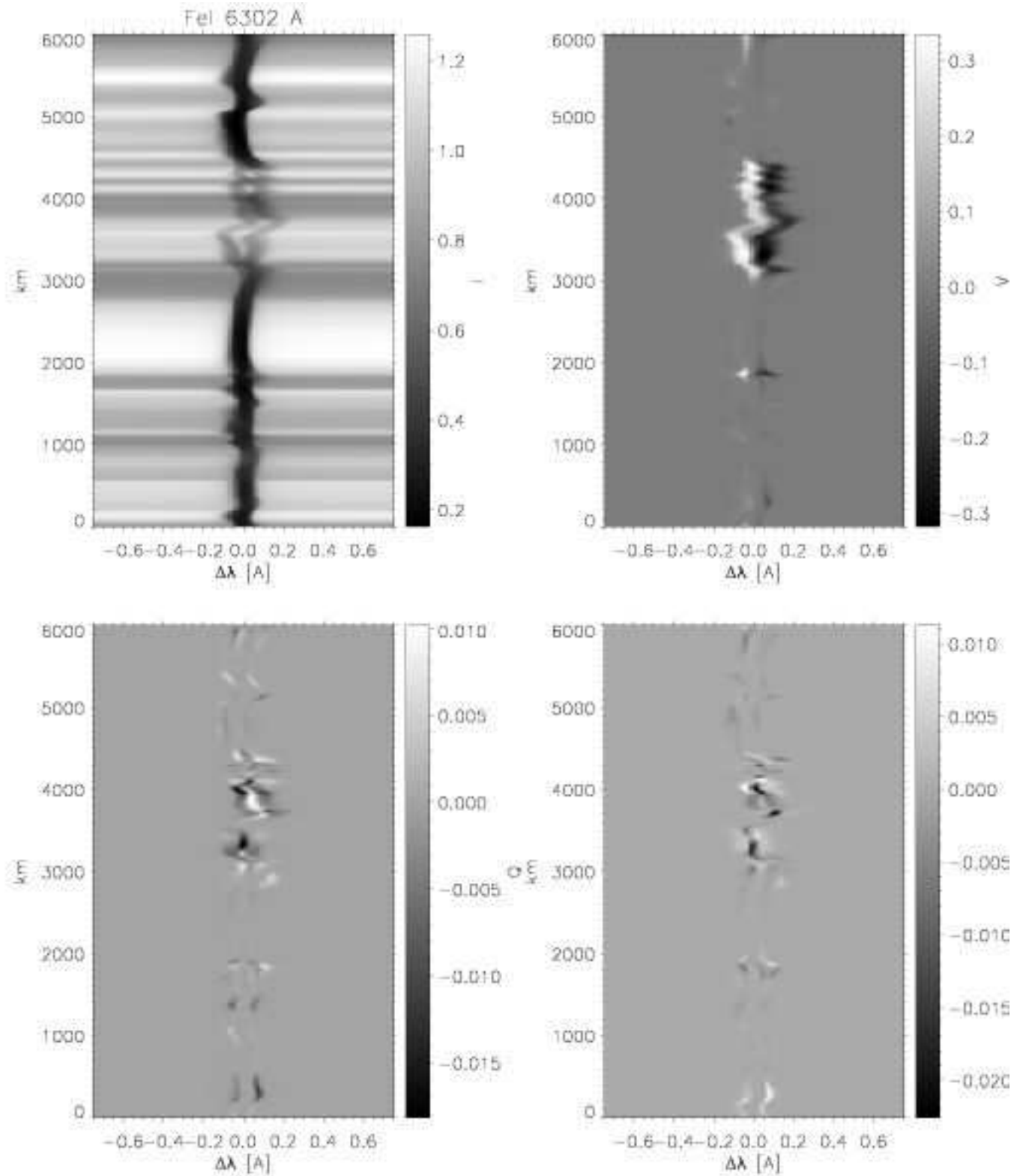
Fig. 5. Synthetic slit spectra, calculated for the 630.2 nm line. Top left: Stokes- I , top right: Stokes- V/I , bottom left: Stokes- Q/I , bottom right: Stokes- U/I . The position of the slit is indicated by the vertical line in the top left panel of Fig. 3.
