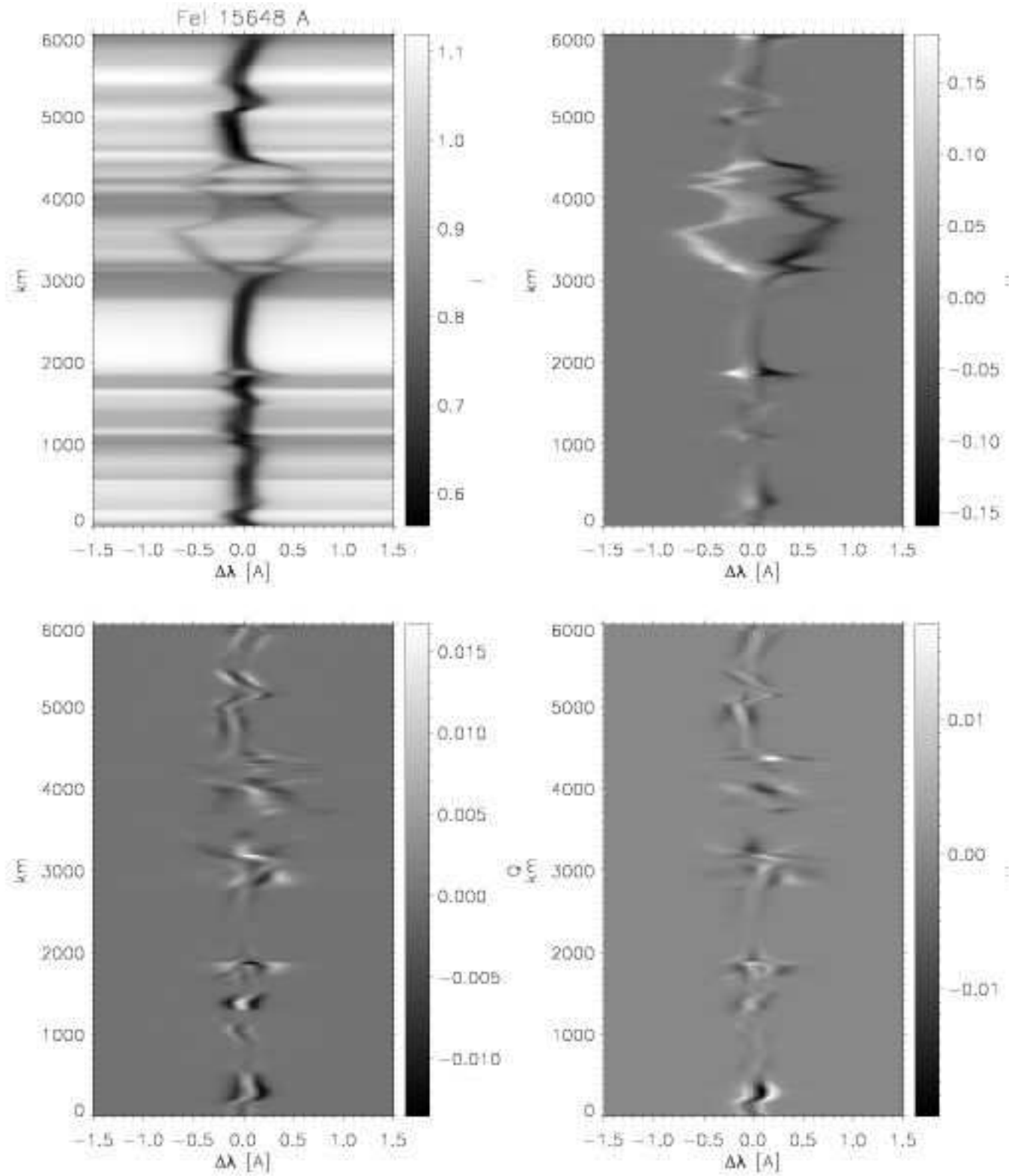
Fig. 6. Same as Fig. 5 for the 1564.8 nm line.
