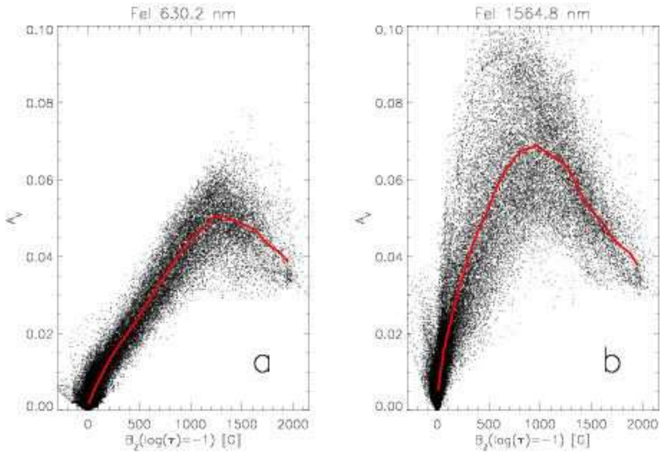
Fig. 14. Scatter plots of the unsigned Stokes- V area versus the vertical (line-of-sight) component of the magnetic field at \tau_{500} = 0.1 a : Fe I 630.2 nm, b : Fe I 1564.8 nm. The lines show binned averages.
