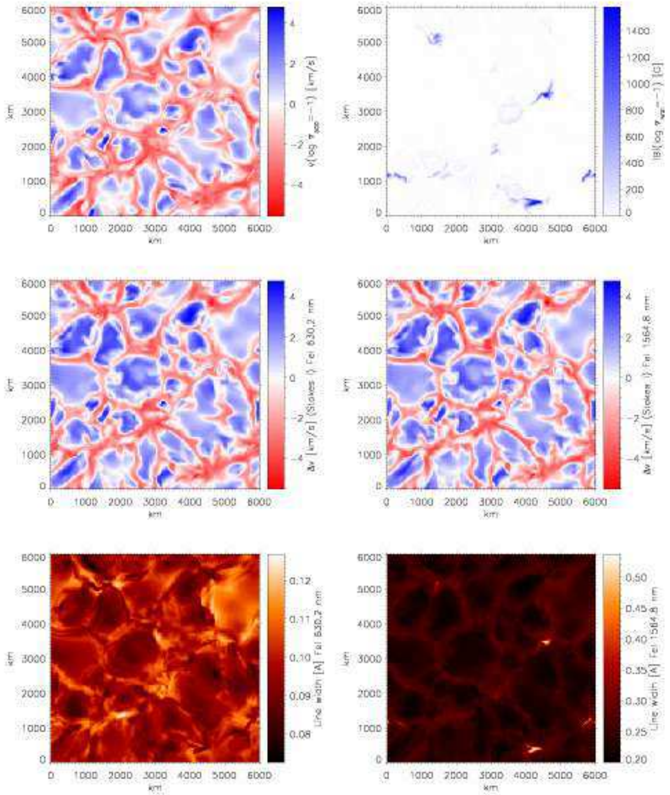
Fig. 8. Same as Fig. 7 for the \langle B_z \rangle = 10\text{ G} simulation.
