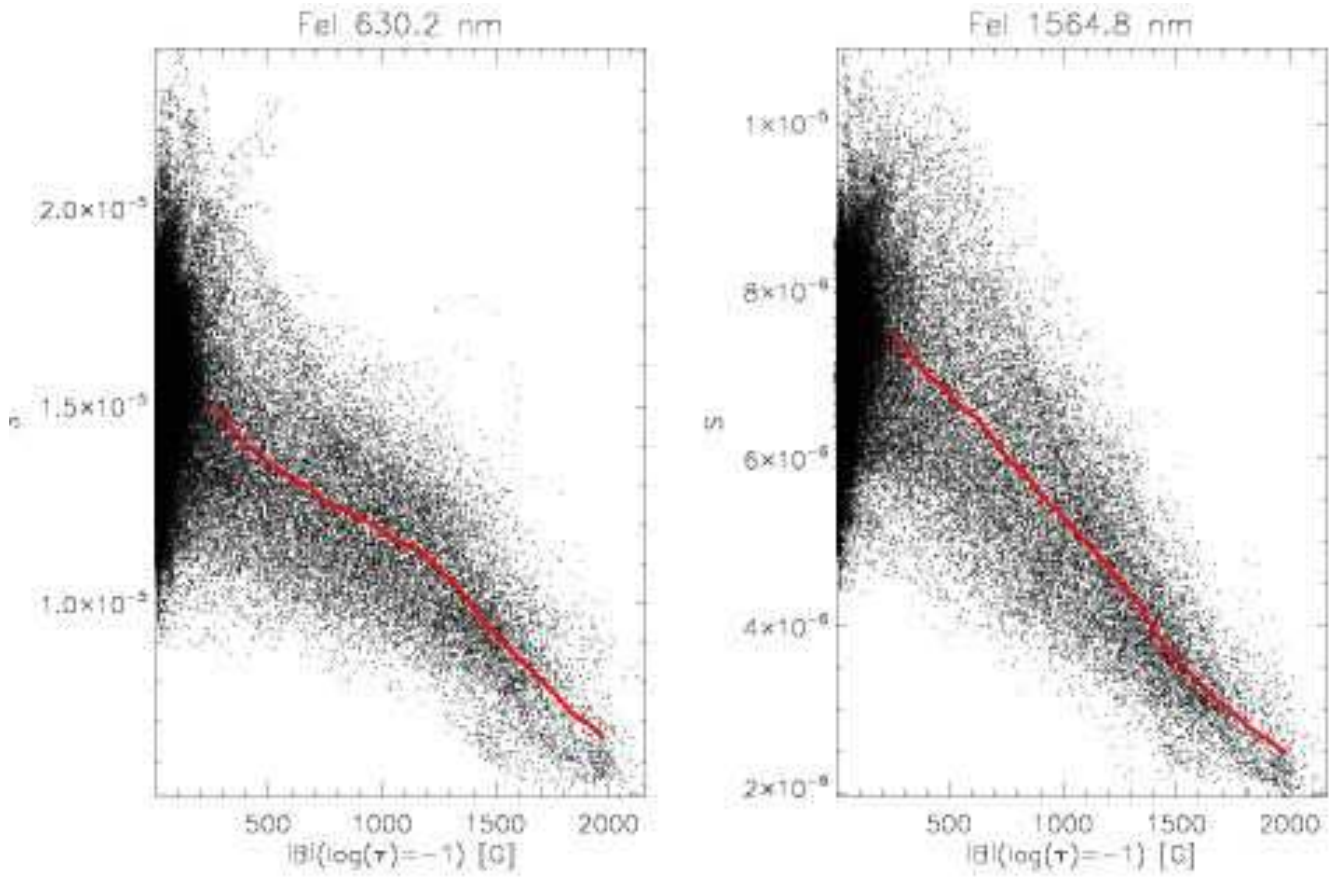
Fig. 12. Scatter plots of line strength versus magnetic field strength at \tau_{500} = 0.1 for the snapshot from the \langle B_z \rangle = 200 G simulation. a : Fe I 630.2 nm, b : Fe I 1564.8 nm. The lines show the binned averages. Note the different vertical scales on the two panels.
