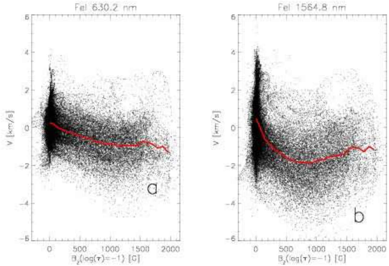
Fig. 20. Scatter plots of the line-of-sight velocity calculated from the zero-crossing-wavelength of the Stokes- V profile versus the vertical component of the magnetic field at \tau_{500} = 0.1 . a : Fe I 630.2 nm, b : Fe I 1564.8 nm. The lines show binned averages. On average, strong magnetic flux concentrations are associated with downflows (negative velocity), while weak fields B < 200 G show some preference for (granular) upflows.
