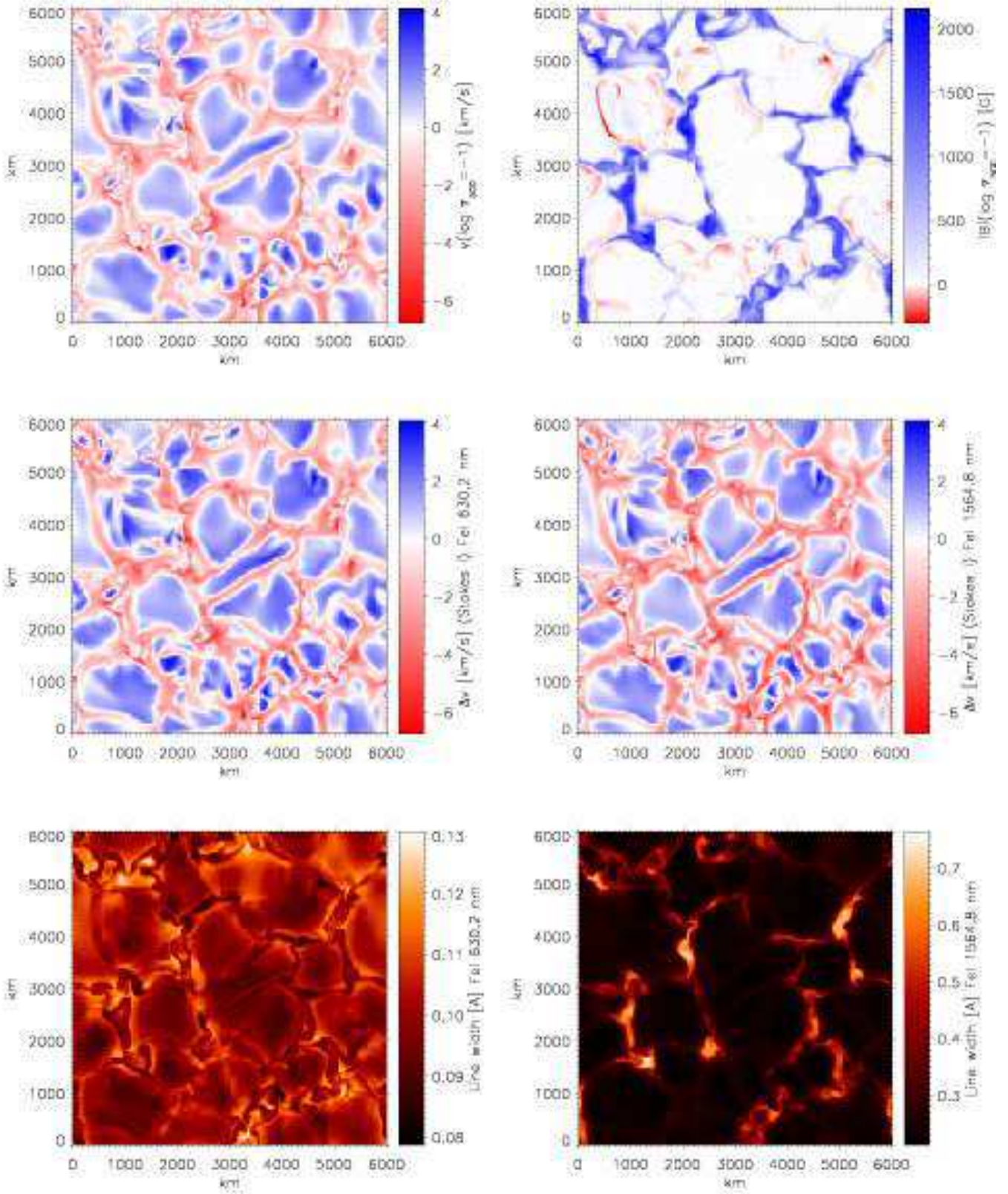
Fig. 7. Vertical velocity (top left panel) and field strength (top right panel) at the surface \tau_{500} = 0.1 for the \langle B_z \rangle = 200\text{ G} simulation. The middle row shows maps of the vertical velocity as determined from the Doppler shift of the 630.2 nm line (middle left panel) and the 1564.8 nm line (middle right panel). The bottom row gives maps of the line width of the 630.2 nm line (bottom left panel) and the 1564.8 nm line (bottom right panel).
