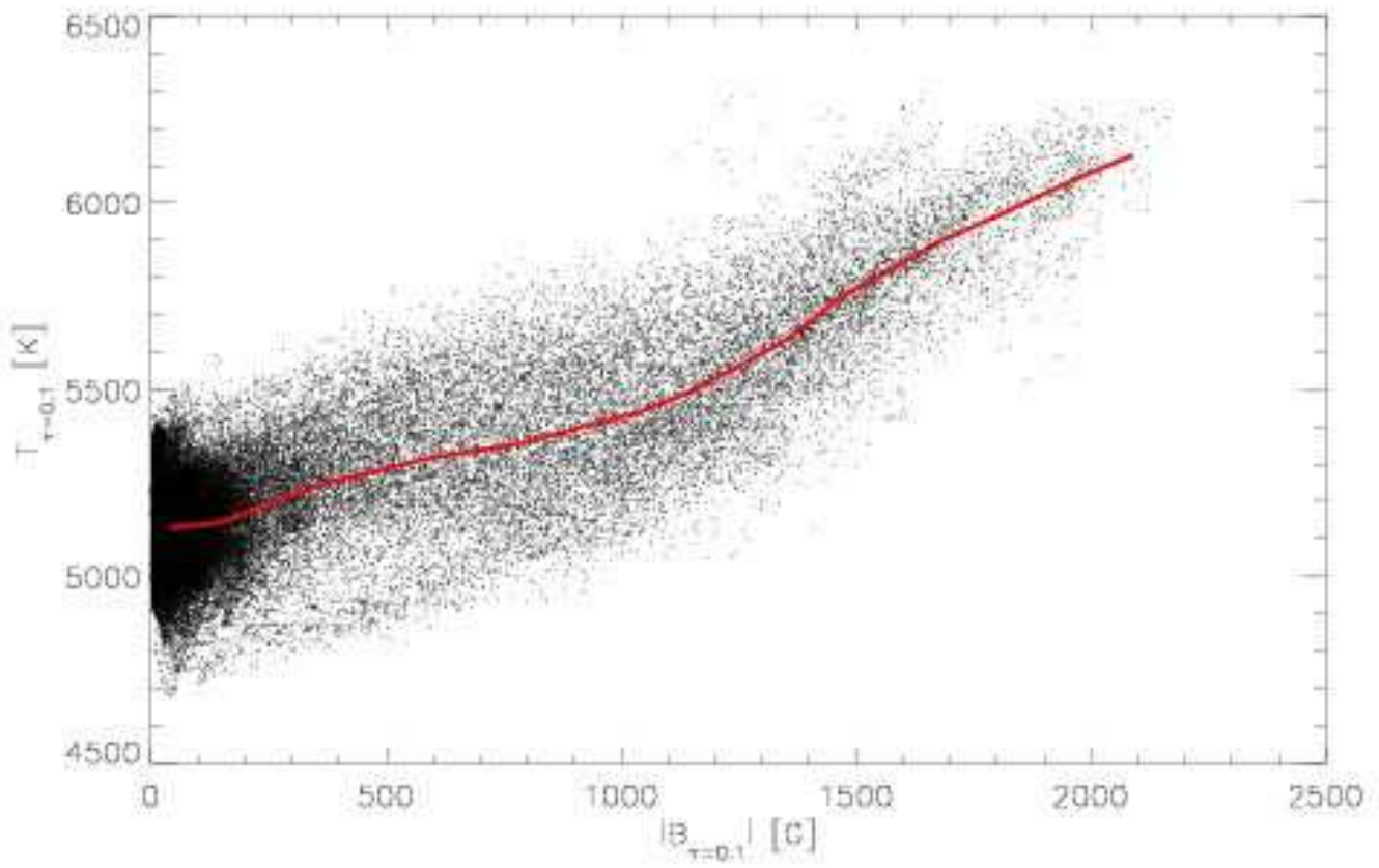
Fig. 13. Scatter plots of temperature versus magnetic field strength (both at \tau_{500} = 0.1 ). The line shows the binned average.
