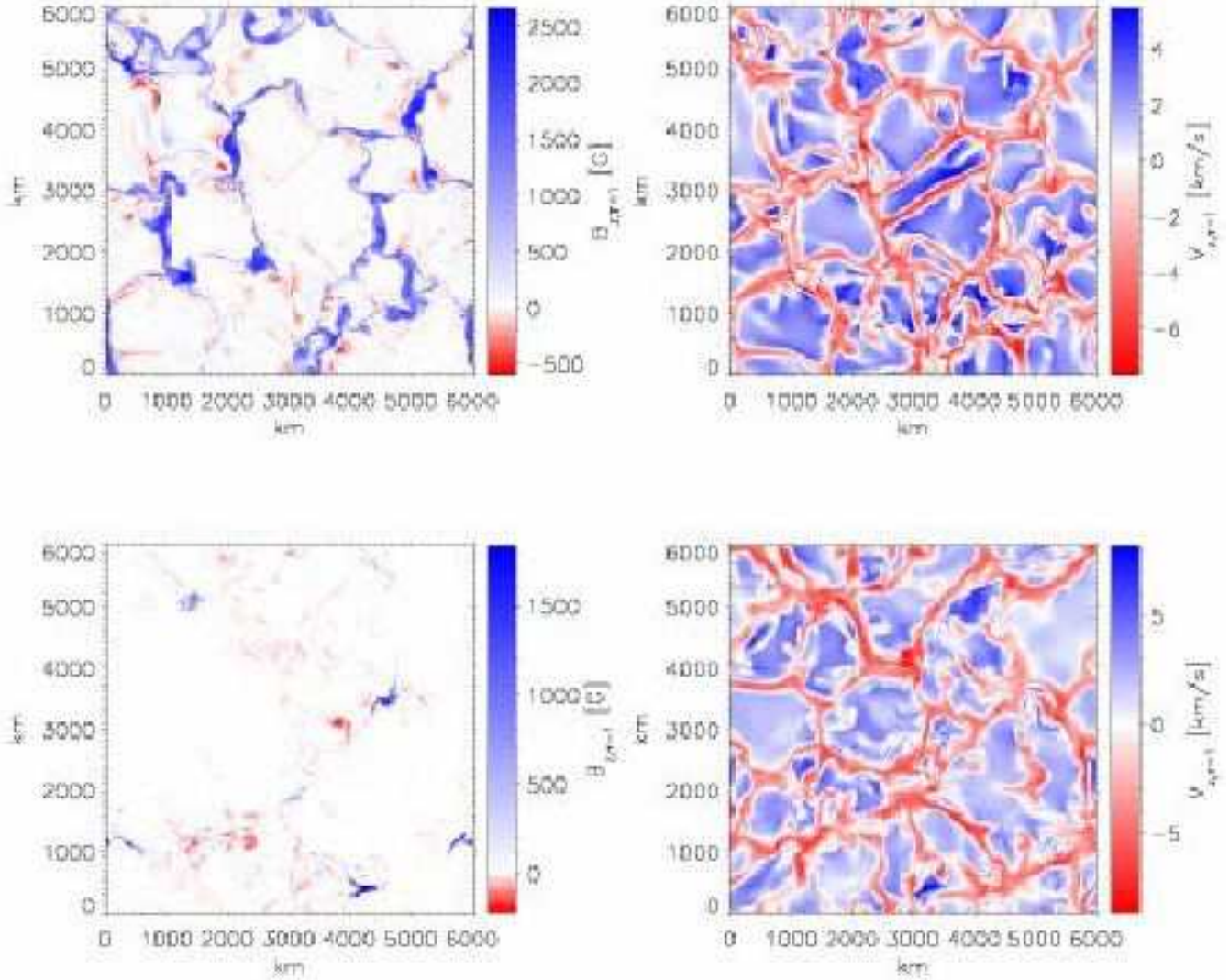
Fig. 1. Vertical magnetic field component (left panels) and vertical velocity (right panels) on the surface \tau_{500} = 1 (continuum optical depth unity at 500 nm wavelength) for snapshots from simulations with \langle B_z \rangle = 200\text{ G} (plage, upper row) and \langle B_z \rangle = 10\text{ G} (decay phase, bottom row). Positive values of the velocity (shown in blue) correspond to upflows; downflows are indicated in red. Note the different scales for positive and negative B_z in the left panel (all negative-polarity field is rather weak).
