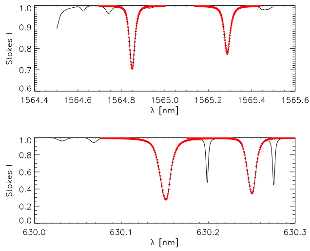
Fig. 2. Comparison between the spatially averaged synthetic Fe I line profiles for the simulation with \langle B_z \rangle = 10 G (diamond symbols) and observed quiet-Sun profiles (solid curves) from the spectral atlas of Delbouille et al. (1973).
