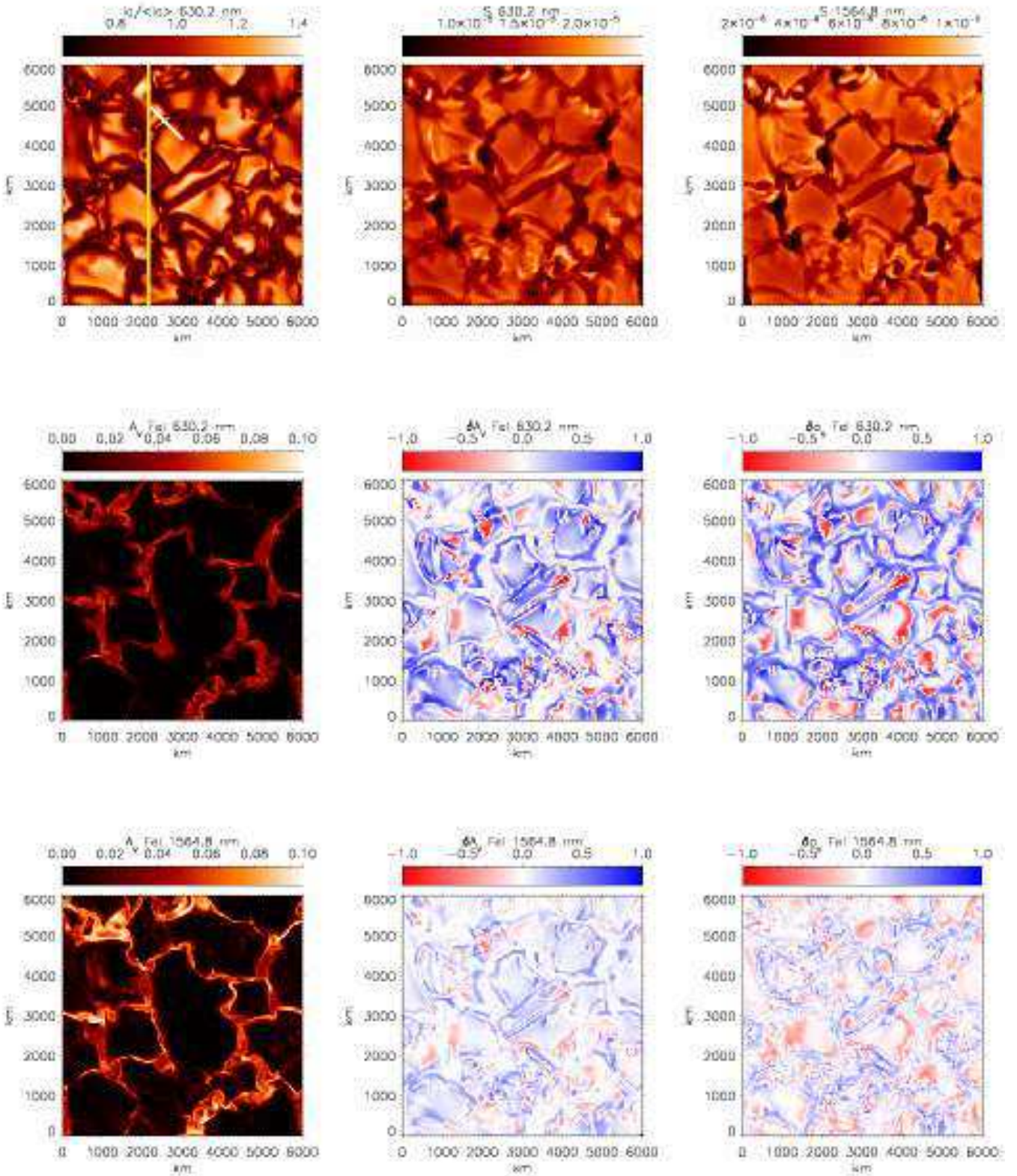
Fig. 3. Properties of synthetic Stokes- I and Stokes- V profiles for the snapshot from the \langle B_z \rangle = 200 G simulation shown in Fig. 1. Given are maps of the (normalized) continuum intensity at 630.2 nm (top left panel), line strength, S (top middle panel for Fe I 630.2 nm and top right panel for Fe I 1564.8 nm), unsigned Stokes- V area, A_V (middle left panel for 630.2 nm and bottom left panel for 1564.8 nm), Stokes- V area asymmetry (central panel for 630.2 nm and bottom middle panel for 1564.8 nm), and Stokes- V amplitude asymmetry (middle right panel for 630.2 nm and bottom right panel for 1564.8 nm). In the continuum intensity image (top left panel), the slit position for Figs. 6 and 5 is indicated by the vertical line and the cut through the magnetic flux sheet shown in Fig. 10 is indicated by the inclined line in the upper left quadrant.
