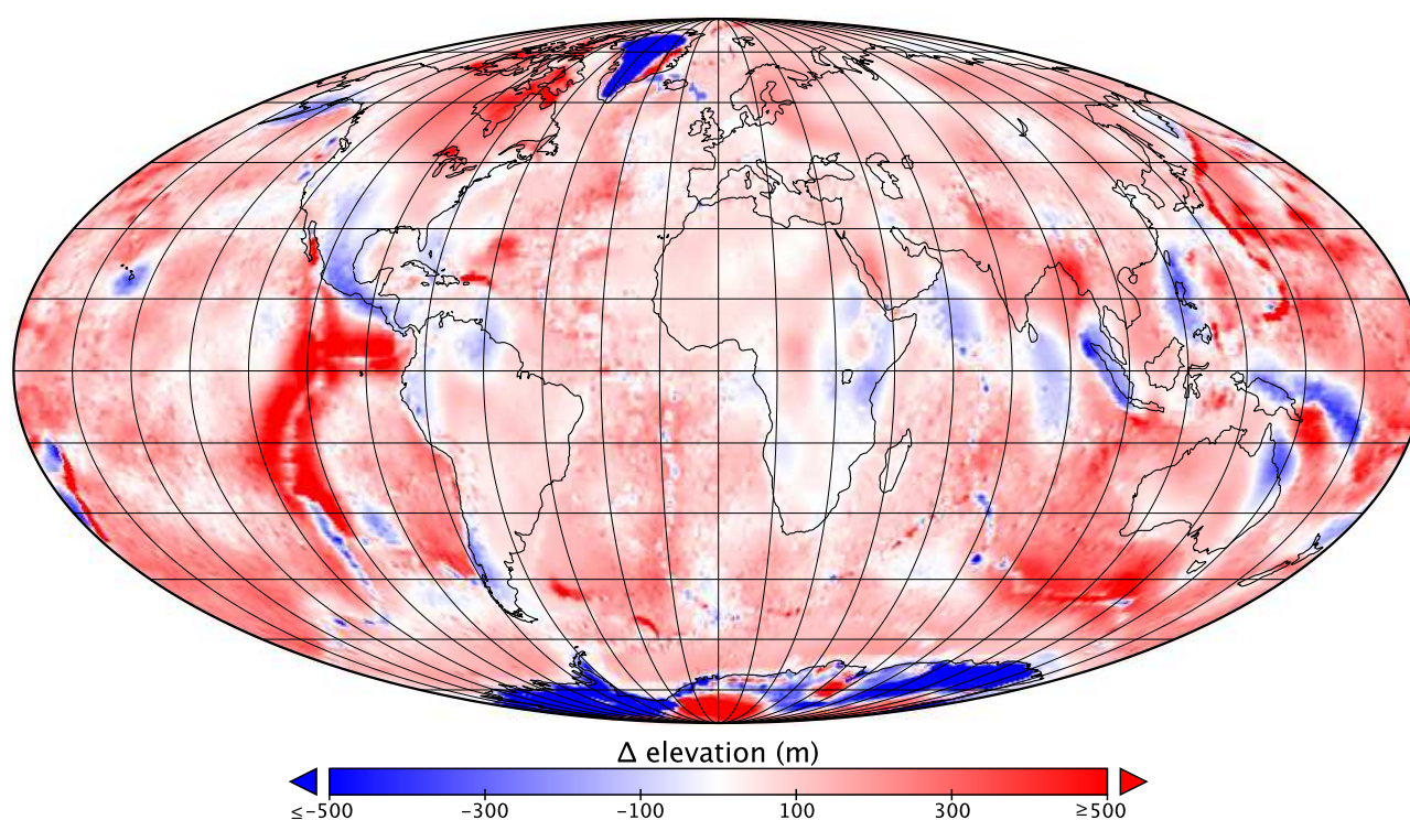
Figure 7: PRISM4 palaeogeographic anomaly showing Piacenzian elevation minus modern (ETOPO1) elevations (red positive, blue negative).
