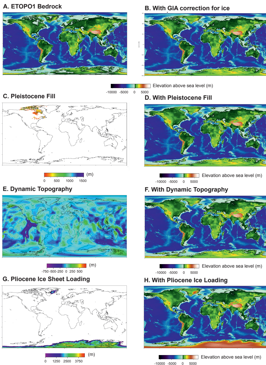
5 Figure 4: Generation of the PRISM4 palaeogeography. (A) shows ‘bedrock’ (base of the ice sheets) version of ETOPO1 sampled at the working resolution of a quarter degree; (B) GIA correction; (C) Pleistocene landscape fill; (D) Pleistocene landscape features filled in; (E) dynamic topography correction; (F) Dynamic topography correction applied to (D); (G) Piacenzian ice sheets; (H) Retrodicted PRISM4 palaeogeography ((G) applied to (F)).
