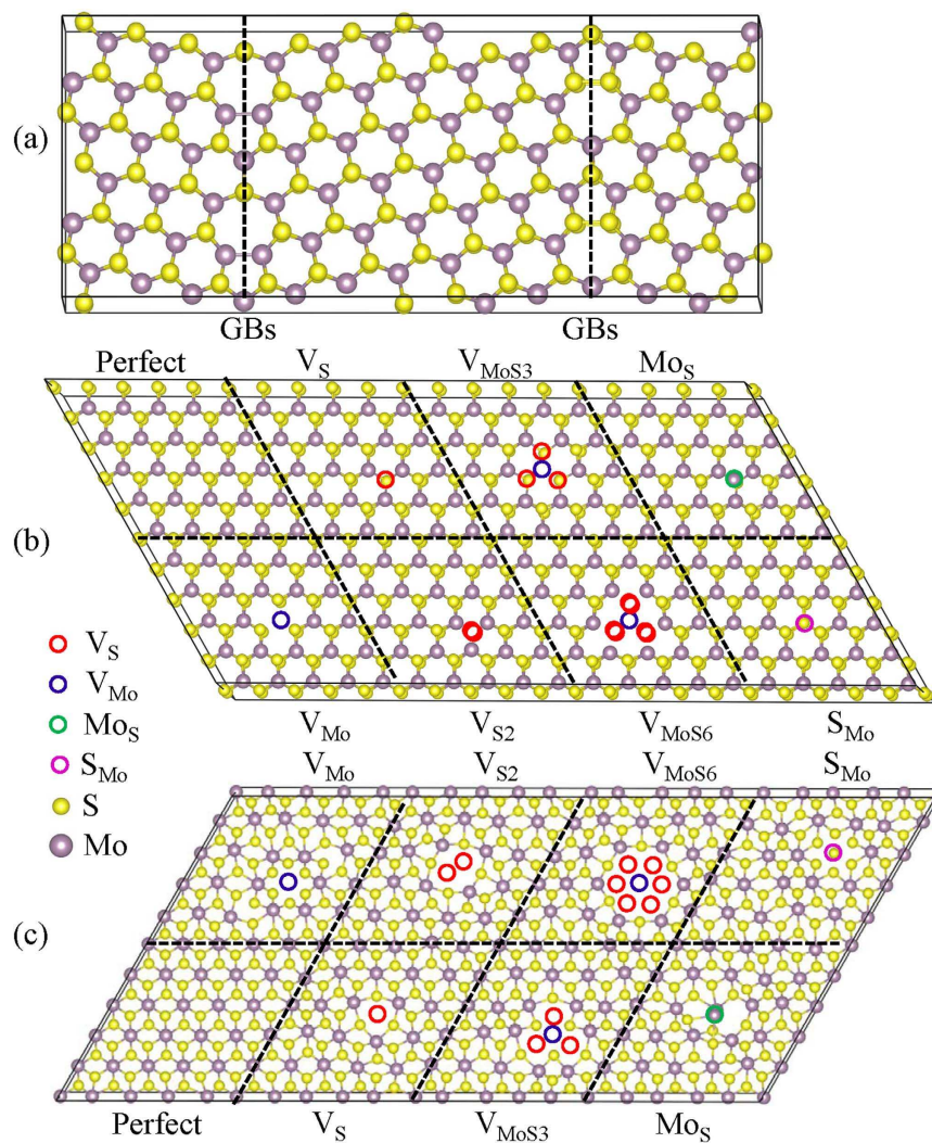
Figure 1. Atomistic configuration of MoS 2 with defects. Optimized atomistic configurations of (a) grain boundary and defects including V Mo , V S , V S 2 , V MoS 3 , V MoS 6 , S Mo in (b) 2H-MoS 2 and (c) 1T-MoS 2 monolayers.
