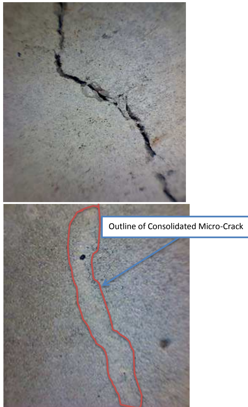
Figure 3 – Above cracked fibre beam and below MICP sealing the crack
