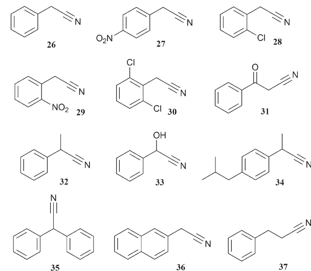
Fig. 2 Nitrile substrates used to screen each nitrilase CFE.
