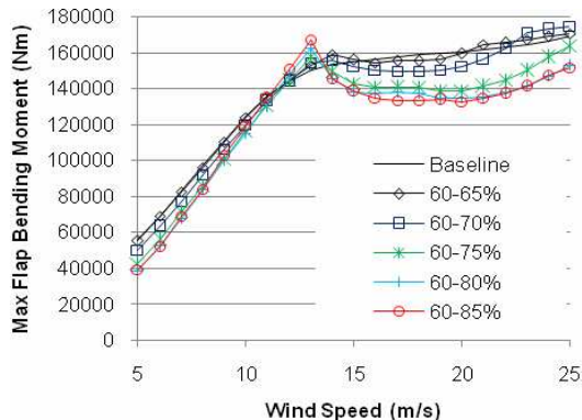
Figure-10. Effect of flap size on flap bending moment at the root of the blade.
